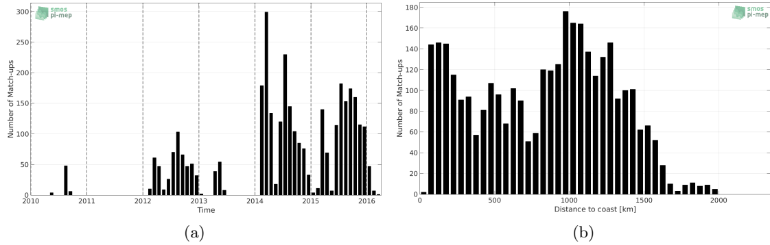
Figure 1: Number of match-ups between Sea mammals and SMOS-L3-CATDS-CECOS-IFREMER-V2-1DAY-0.5DEG SSS as a function of time (a) and as function of the distance to coast (b) over the Pacific Ocean Pi-MEP region and for the full satellite product period.
