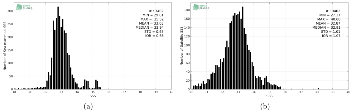
Figure 2: Histograms of SSS from Sea mammals (a) and SMOS-L3-CATDS-CECOS-IFREMER-V2-1DAY-0.5DEG (b) considering all match-up pairs per bins of 0.1 over the Pacific Ocean Pi-MEP region and for the full satellite product period.
