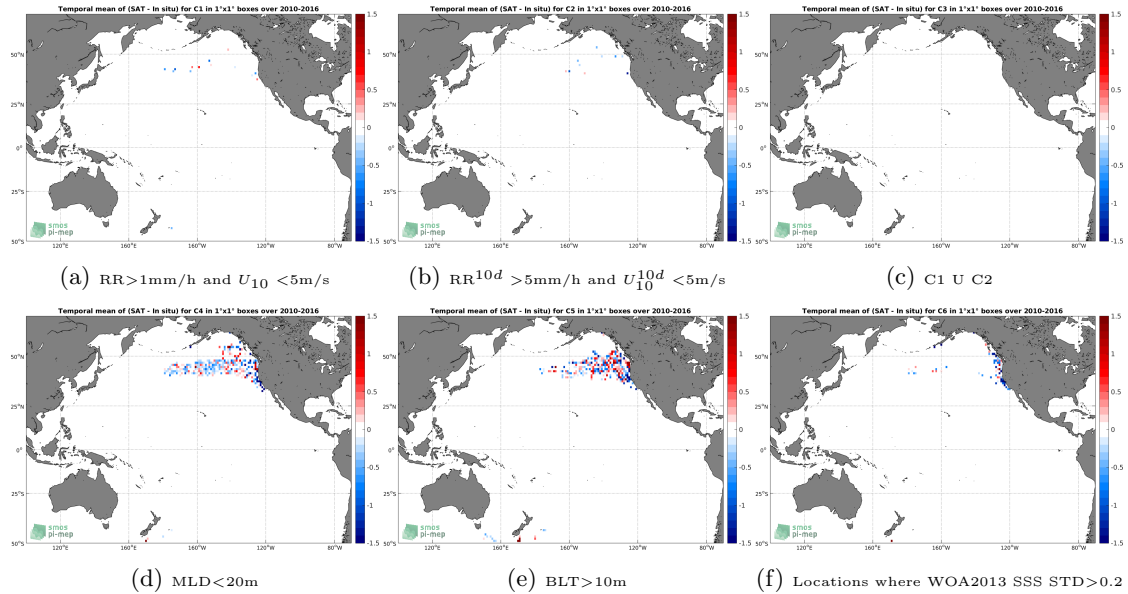
Figure 12: Temporal mean gridded over spatial boxes of size 1^\circ \times 1^\circ of \Delta\text{SSS} (SMOS-L3-CATDS-CECOS-IFREMER-V2-1DAY-0.5DEG - Sea mammals) for 6 different subdatasets corresponding to: RR > 1\text{mm/h} and U_{10} < 5\text{m/s} (a), RR^{10d} > 5\text{mm/h} and U_{10}^{10d} < 5\text{m/s} (b), C1 U C2 (c), \text{MLD} < 20\text{m} (d), \text{BLT} > 10\text{m} (e), Locations where WOA2013 SSS STD > 0.2 (f).
