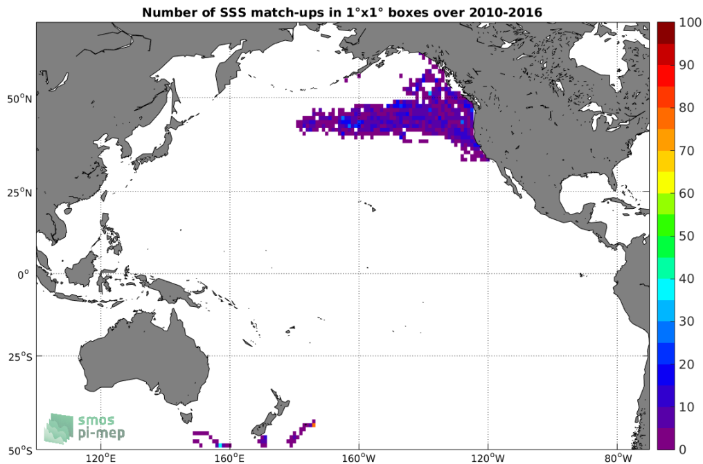
Figure 4: Number of SSS match-ups between Sea mammals SSS and the SMOS-L3-CATDS-CECOS-IFREMER-V2-1DAY-0.5DEG SSS product for the Pacific Ocean Pi-MEP region over 1°x1° boxes and for the full satellite product period.
