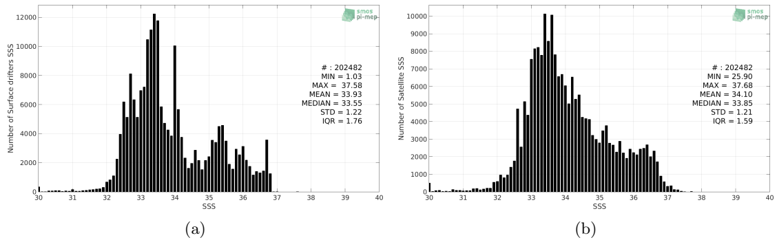
Figure 2: Histograms of SSS from Surface drifters (a) and SMOS SSS L3 v2 - Daily - 0.5 Deg (CATDS-CECOS-IFREMER) (b) considering all match-up pairs per bins of 0.1 over the Pacific Ocean Pi-MEP region and for the full satellite product period.
