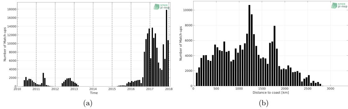
Figure 1: Number of match-ups between Surface drifters and SMOS SSS L3 v2 - Daily - 0.5 Deg (CATDS-CECOS-IFREMER) SSS as a function of time (a) and as function of the distance to coast (b) over the Pacific Ocean Pi-MEP region and for the full satellite product period.
