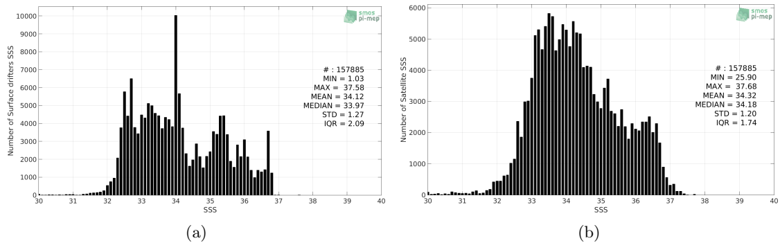
Figure 2: Histograms of SSS from Surface drifters (a) and SMOS L3 v2 - Daily - 0.5 Deg (CATDS-CECOS-IFREMER) (b) considering all match-up pairs per bins of 0.1 over the Pacific Ocean Pi-MEP region and for the full satellite product period.
