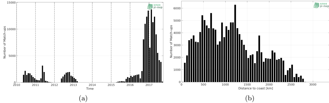
Figure 1: Number of match-ups between Surface drifters and SMOS L3 v2 - Daily - 0.5 Deg (CATDS-CECOS-IFREMER) SSS as a function of time (a) and as function of the distance to coast (b) over the Pacific Ocean Pi-MEP region and for the full satellite product period.
