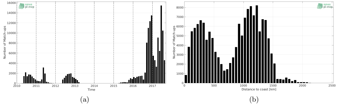
Figure 1: Number of match-ups between Surface drifters and SMOS-L3-CATDS-CECOS-IFREMER-V2-1DAY-0.5DEG SSS as a function of time (a) and as function of the distance to coast (b) over the Pacific Ocean Pi-MEP region and for the full satellite product period.
