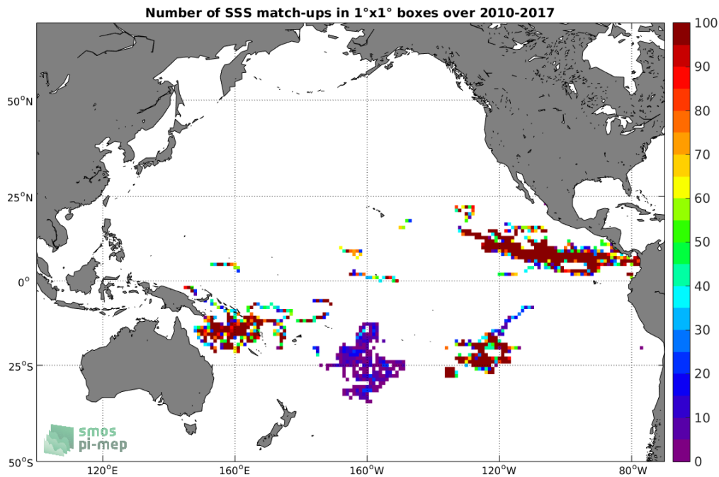
Figure 3: Number of SSS match-ups between Surface drifters SSS and the SMOS-L3-CATDS-CECOS-IFREMER-V2-1DAY-0.5DEG SSS product for the Pacific Ocean Pi-MEP region over 1^\circ \times 1^\circ boxes and for the full satellite product period.
