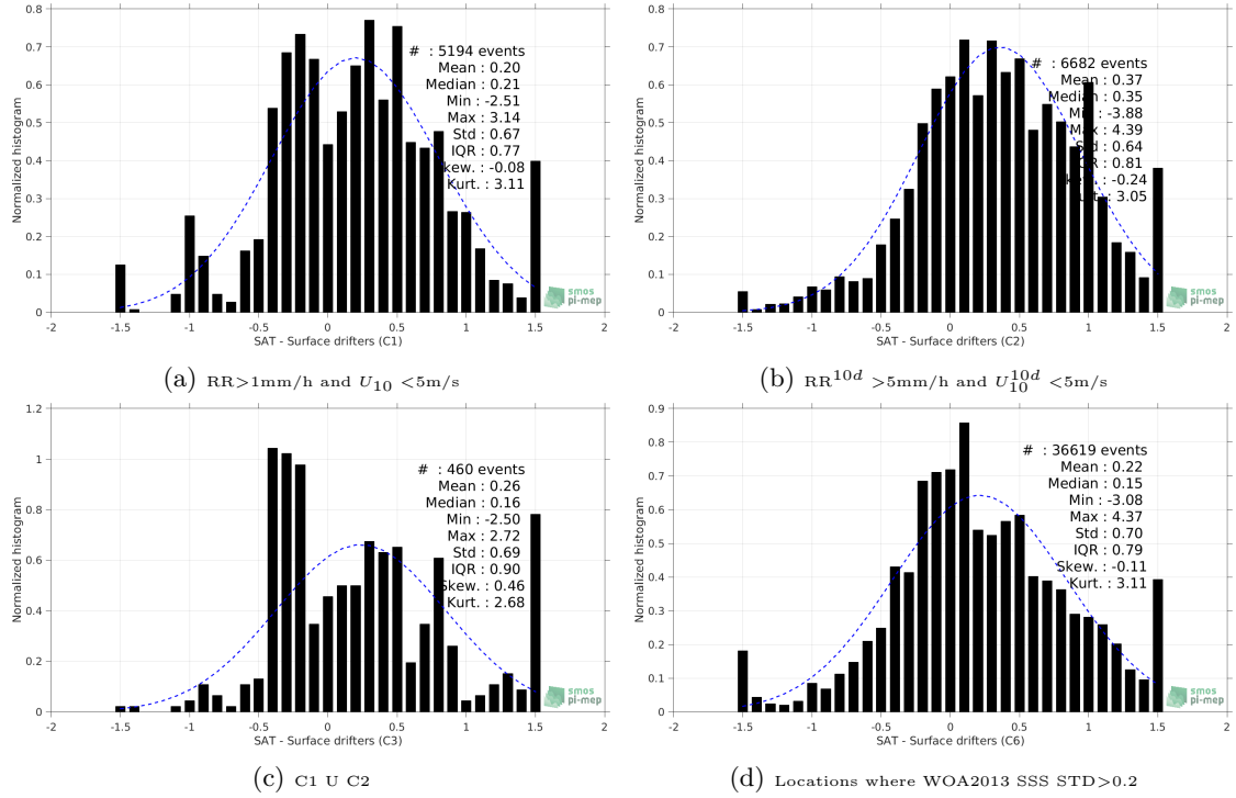
Figure 12: Normalized histogram of \Delta\text{SSS} (SMOS-L3-CATDS-CECOS-IFREMER-V2-1DAY-0.5DEG - Surface drifters) for 6 different subdatasets corresponding to: RR > 1mm/h and U_{10} < 5\text{m/s} (a), RR^{10d} > 5\text{mm/h} and U_{10}^{10d} < 5\text{m/s} (b), C1 U C2 (c), Locations where WOA2013 SSS STD > 0.2 (d).
