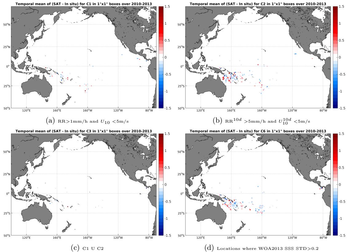
Figure 11: Temporal mean gridded over spatial boxes of size 1^\circ \times 1^\circ of \Delta SSS (SMOS-L3-CATDS-CECOS-IFREMER-V2-1DAY-0.5DEG - Surface drifters) for 4 different subdatasets corresponding to: RR > 1\text{mm/h} and U_{10} < 5\text{m/s} (a), RR^{10d} > 5\text{mm/h} and U_{10}^{10d} < 5\text{m/s} (b), C1 U C2 (c), Locations where WOA2013 SSS STD > 0.2 (d).
