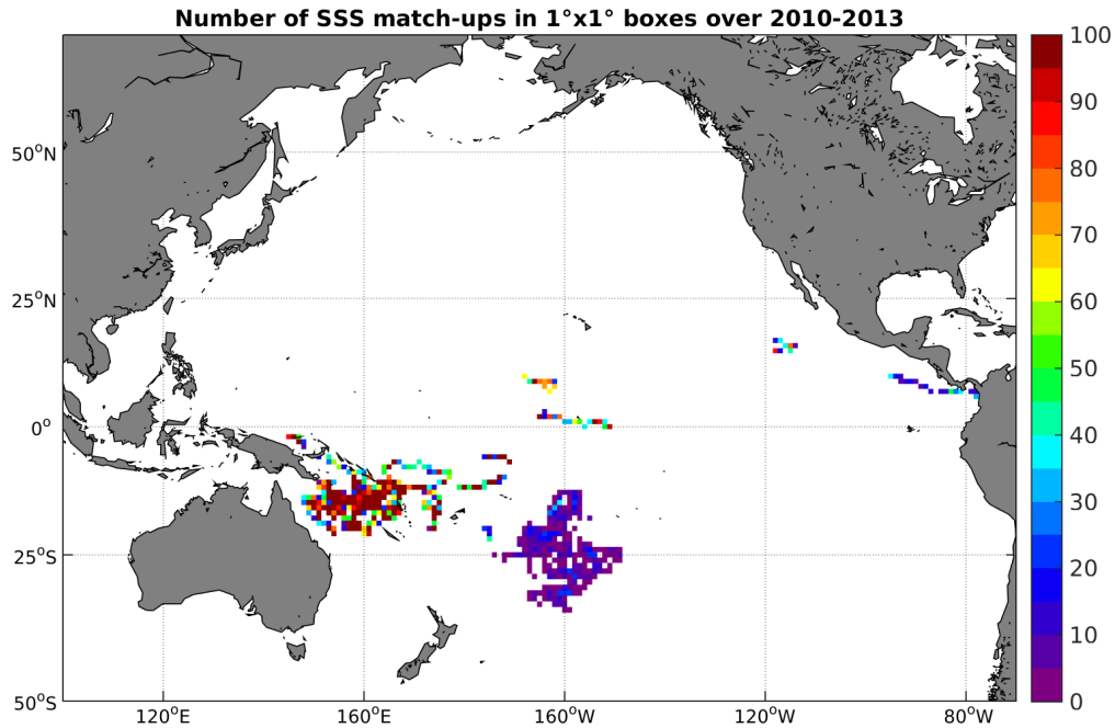
Figure 3: Number of SSS match-ups between Surface drifters SSS and the SMOS-L3-CATDS-CECOS-IFREMER-V2-1DAY-0.5DEG SSS product for the Pacific Ocean Pi-MEP region over 1°x1° boxes and for the full satellite product period.
