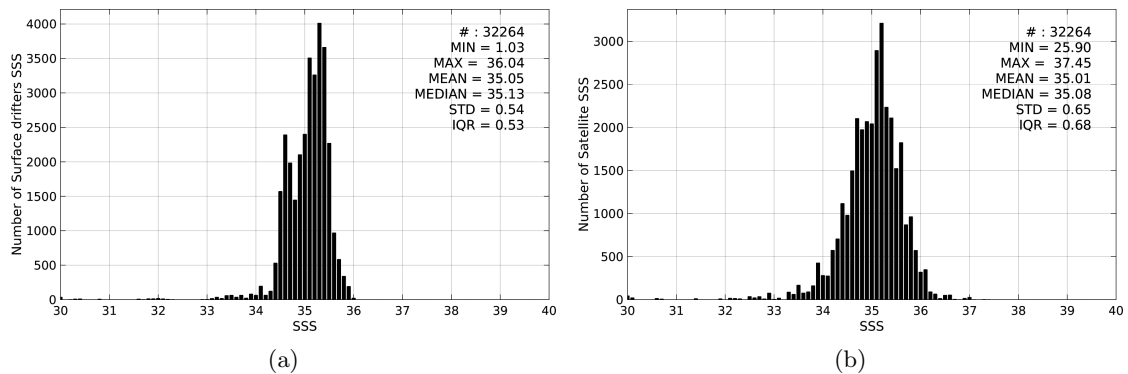
Figure 2: Histograms of SSS from Surface drifters (a) and SMOS-L3-CATDS-CECOS-IFREMER-V2-1DAY-0.5DEG (b) considering all match-up pairs per bins of 0.1 over the Pacific Ocean Pi-MEP region and for the full satellite product period.
