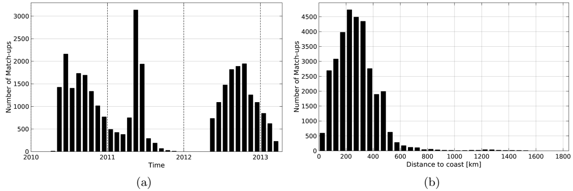
Figure 1: Number of match-ups between Surface drifters and SMOS-L3-CATDS-CECOS-IFREMER-V2-1DAY-0.5DEG SSS as a function of time (a) and as function of the distance to coast (b) over the Pacific Ocean Pi-MEP region and for the full satellite product period.
