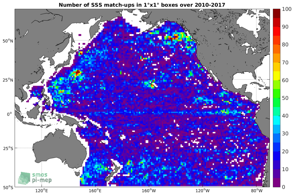
Figure 4: Number of SSS match-ups between Argo SSS and the SMOS L3 v2 - Daily - 0.5 Deg (CATDS-CECOS-IFREMER) SSS product for the Pacific Ocean Pi-MEP region over 1^\circ \times 1^\circ boxes and for the full satellite product period.
