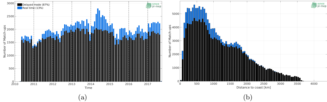
Figure 1: Number of match-ups between Argo and SMOS L3 v2 - Daily - 0.5 Deg (CATDS-CECOS-IFREMER) SSS as a function of time (a) and as function of the distance to coast (b) over the Pacific Ocean Pi-MEP region and for the full satellite product period.
