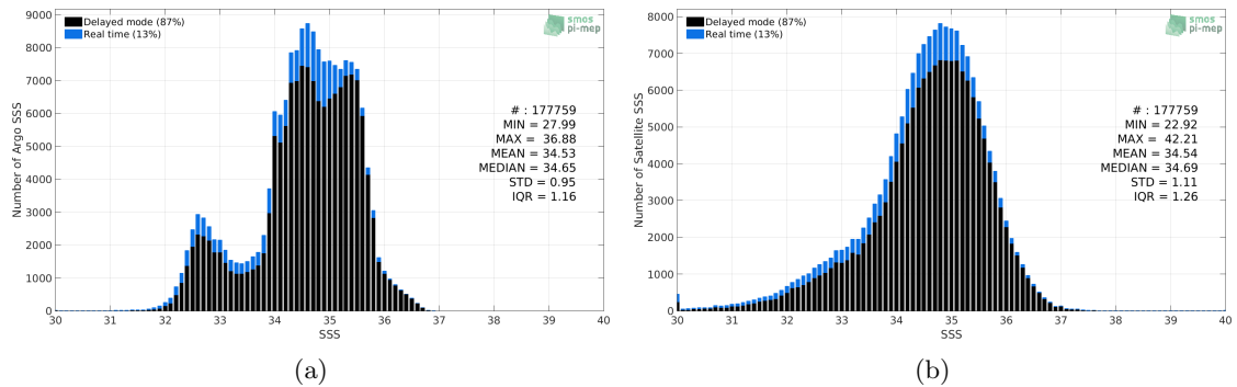
Figure 2: Histograms of SSS from Argo (a) and SMOS L3 v2 - Daily - 0.5 Deg (CATDS-CECOS-IFREMER) (b) considering all match-up pairs per bins of 0.1 over the Pacific Ocean Pi-MEP region and for the full satellite product period.
