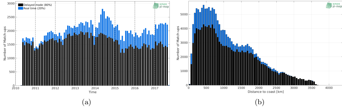
Figure 1: Number of match-ups between Argo and SMOS-L3-CATDS-CECOS-IFREMER-V2-1DAY-0.5DEG SSS as a function of time (a) and as function of the distance to coast (b) over the Pacific Ocean Pi-MEP region and for the full satellite product period.
