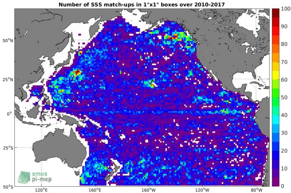
Figure 4: Number of SSS match-ups between Argo SSS and the SMOS-L3-CATDS-CECOS-IFREMER-V2-1DAY-0.5DEG SSS product for the Pacific Ocean Pi-MEP region over 1^\circ \times 1^\circ boxes and for the full satellite product period.
