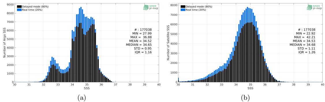
Figure 2: Histograms of SSS from Argo (a) and SMOS-L3-CATDS-CECOS-IFREMER-V2-1DAY-0.5DEG (b) considering all match-up pairs per bins of 0.1 over the Pacific Ocean Pi-MEP region and for the full satellite product period.
