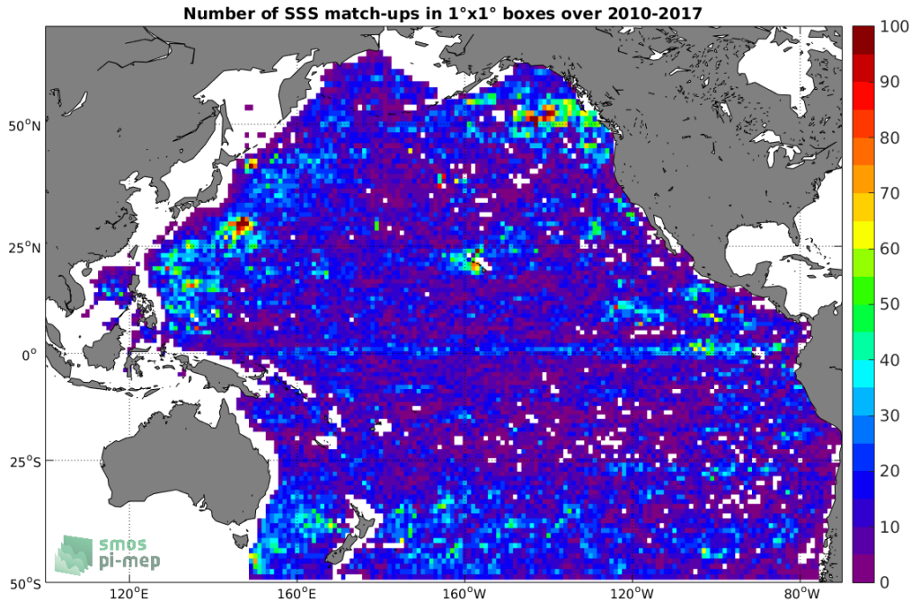
Figure 4: Number of SSS match-ups between Argos SSS and the SMOS-L3-CATDS-CECOS-IFREMER-V2-1DAY-0.5DEG SSS product for the Pacific Ocean Pi-MEP region over 1^\circ \times 1^\circ boxes and for the full satellite product period.
