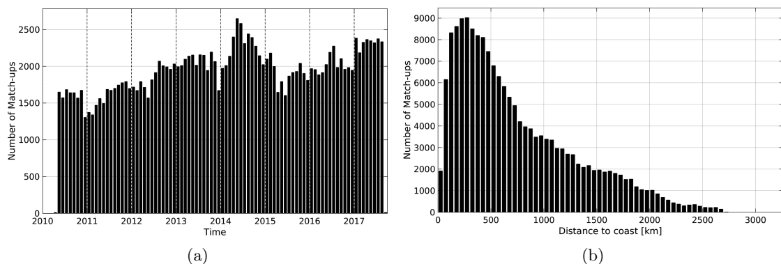
Figure 1: Number of match-ups between Argo and SMOS-L3-CATDS-CECOS-IFREMER-V2-1DAY-0.5DEG SSS as a function of time (a) and as function of the distance to coast (b) over the Pacific Ocean Pi-MEP region and for the full satellite product period.
