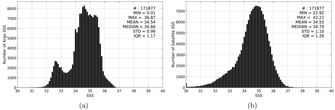
Figure 2: Histograms of SSS from Argo (a) and SMOS-L3-CATDS-CECOS-IFREMER-V2-1DAY-0.5DEG (b) considering all match-up pairs per bins of 0.1 over the Pacific Ocean Pi-MEP region and for the full satellite product period.
