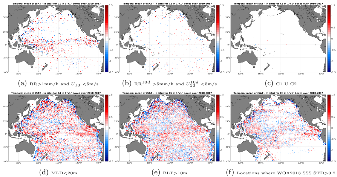
Figure 12: Temporal mean gridded over spatial boxes of size 1^\circ \times 1^\circ of \Delta SSS (SMOS-L3-CATDS-CECOS-IFREMER-V2-1DAY-0.5DEG - Argo) for 6 different subdatasets corresponding to:RR >1 mm/h and U_{10} < 5 m/s (a), RR 10d > 5 mm/h and U_{10}^{10d} < 5 m/s (b), C1 U C2 (c),MLD <20 m (d),BLT >10 m (e),Locations where WOA2013 SSS STD >0.2 (f).
