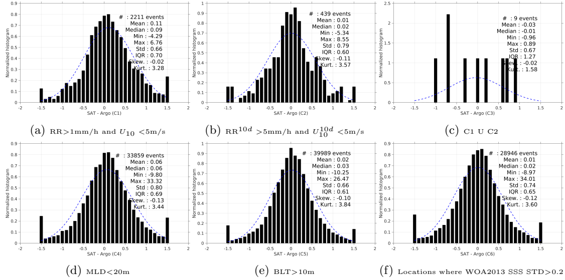
Figure 13: Normalized histogram of \Delta\text{SSS} (SMOS-L3-CATDS-CECOS-IFREMER-V2-1DAY-0.5DEG - Argo) for 6 different subdatasets corresponding to: RR>1mm/h and U_{10} < 5\text{m/s} (a), \text{RR}^{10d} > 5\text{mm/h} and U_{10}^{10d} < 5\text{m/s} (b), C1 U C2 (c),MLD<20m (d),BLT>10m (e),Locations where WOA2013 SSS STD>0.2 (f).
