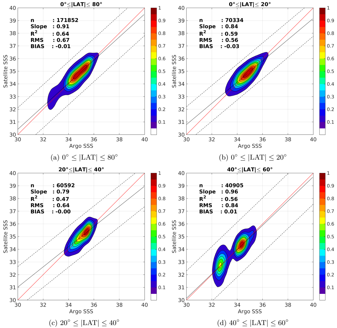
Figure 9: Contour maps of the concentration of SMOS-L3-CATDS-CECOS-IFREMER-V2-1DAY-0.5DEG SSS (y-axis) versus Argo SSS (x-axis) at match-up pairs for different latitude bands. For each plot, the red line shows x=y . The black thin and dashed lines indicate a linear fit through the data cloud and the \pm 95\% confidence levels, respectively. The number match-up pairs n , the slope and R^2 coefficient of the linear fit, the root mean square (RMS) and the mean bias between satellite and in situ data are indicated for each latitude band in each plots.
