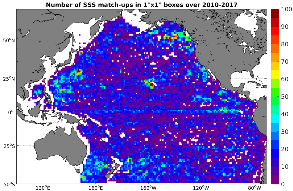
Figure 4: Number of SSS match-ups between Argo SSS and the SMOS-L3-CATDS-CECOS-IFREMER-V2-1DAY-0.5DEG SSS product for the Pacific Ocean Pi-MEP region over 1°x1° boxes and for the full satellite product period.
