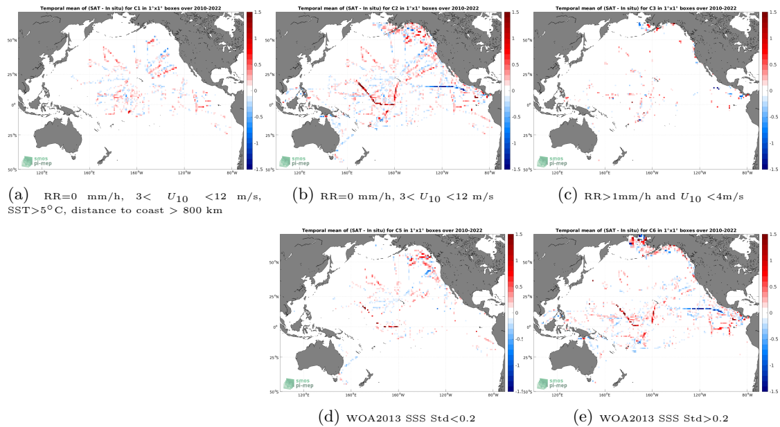
Figure 12: Temporal mean gridded over spatial boxes of size 1^\circ \times 1^\circ of \Delta\text{SSS} (SMOS SSS L3 v335 - Monthly - 25 km (CATDS-CPDC) - TSG (SAMOS)) for 5 different subdatasets corresponding to:RR=0 mm/h, 3 < U_{10} < 12 m/s, SST >5^\circ\text{C} , distance to coast > 800 km (a), RR=0 mm/h, 3 < U_{10} < 12 m/s (b), RR >1 mm/h and U_{10} < 4 m/s (c), WOA2013 SSS Std <0.2 (d), WOA2013 SSS Std >0.2 (e).
