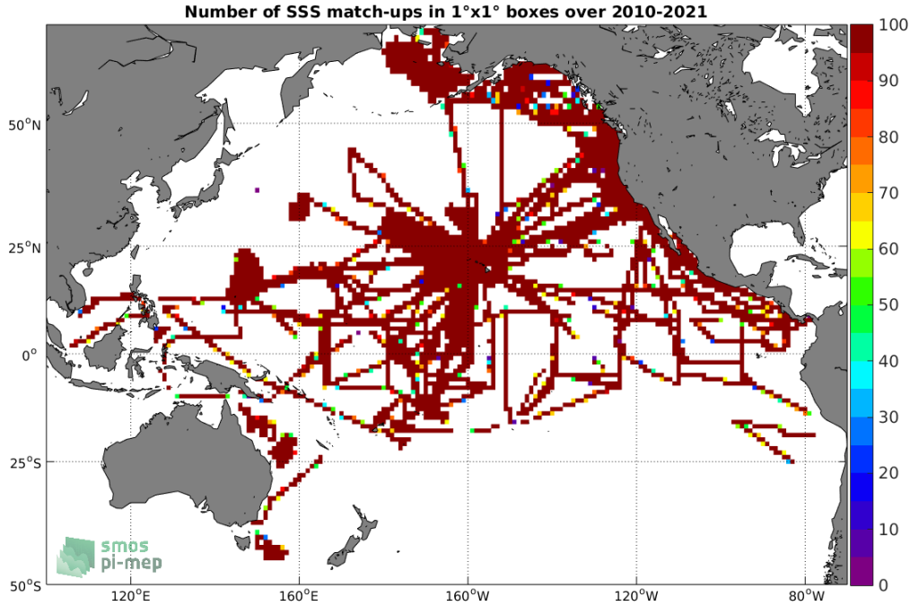
Figure 4: Number of SSS match-ups between TSG (SAMOS) SSS and the SMOS SSS L3 v335 - Monthly - 25 km (CATDS-CPDC) SSS product for the Pacific Ocean Pi-MEP region over 1^\circ \times 1^\circ boxes and for the full satellite product period.
