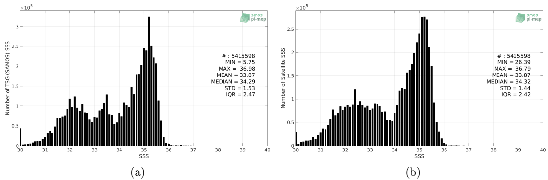
Figure 2: Histograms of SSS from TSG (SAMOS) (a) and SMOS SSS L3 v335 - Monthly - 25 km (CATDS-CPDC) (b) considering all match-up pairs per bins of 0.1 over the Pacific Ocean Pi-MEP region and for the full satellite product period.
