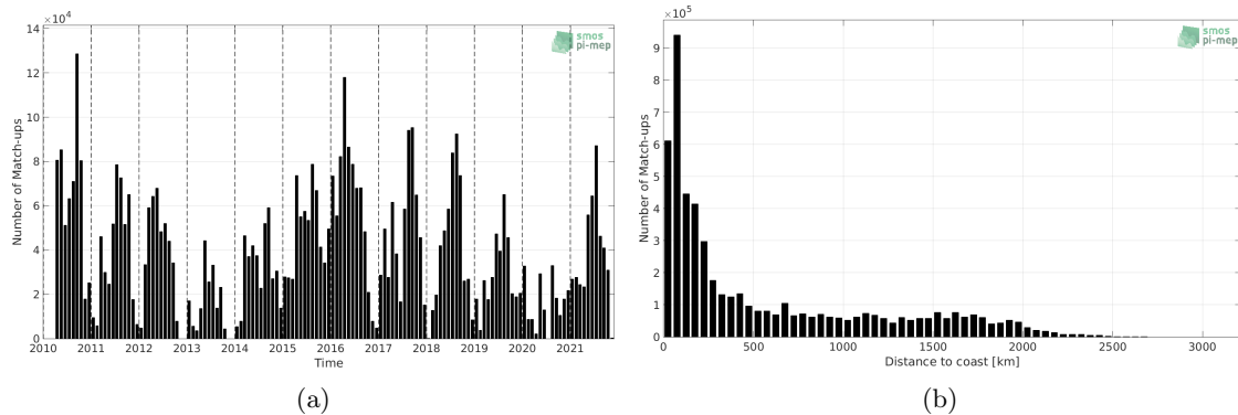
Figure 1: Number of match-ups between TSG (SAMOS) and SMOS SSS L3 v335 - Monthly - 25 km (CATDS-CPDC) SSS as a function of time (a) and as function of the distance to coast (b) over the Pacific Ocean Pi-MEP region and for the full satellite product period.
