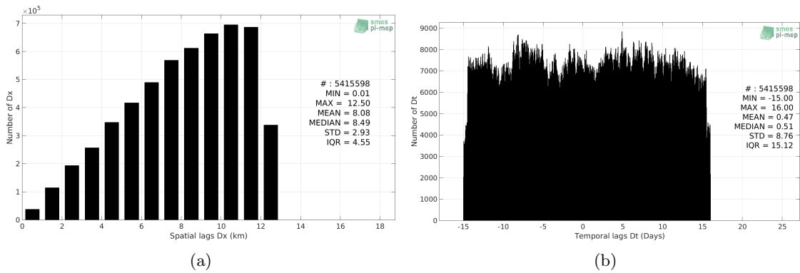
Figure 5: Histograms of the spatial (a) and temporal (b) lags between the location/time of the TSG (SAMOS) measurement and the date of the corresponding SMOS SSS L3 v335 - Monthly - 25 km (CATDS-CPDC) SSS pixel.
