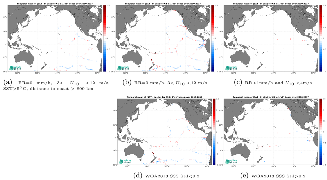
Figure 14: Temporal mean gridded over spatial boxes of size 1^\circ \times 1^\circ of \Delta SSS (SMOS SSS L3 v335 - Monthly - 25 km (CATDS-CPDC) - TSG (GOSUD-Sailing-ship)) for 5 different subdatasets corresponding to:RR=0 mm/h, 3 < U_{10} < 12 m/s, SST >5^\circ\text{C} , distance to coast > 800 km (a), RR=0 mm/h, 3 < U_{10} < 12 m/s (b), RR >1 mm/h and U_{10} < 4 m/s (c), WOA2013 SSS Std <0.2 (d), WOA2013 SSS Std >0.2 (e).
