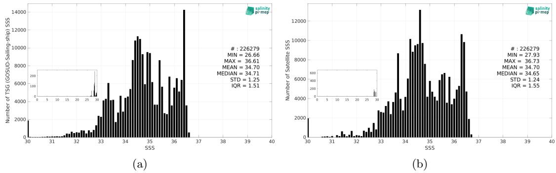
Figure 3: Histograms of SSS from TSG (GOSUD-Sailing-ship) (a) and SMOS SSS L3 v335 - Monthly - 25 km (CATDS-CPDC) (b) considering all match-up pairs per bins of 0.1 over the Pacific Ocean Pi-MEP region and for the full satellite product period.
