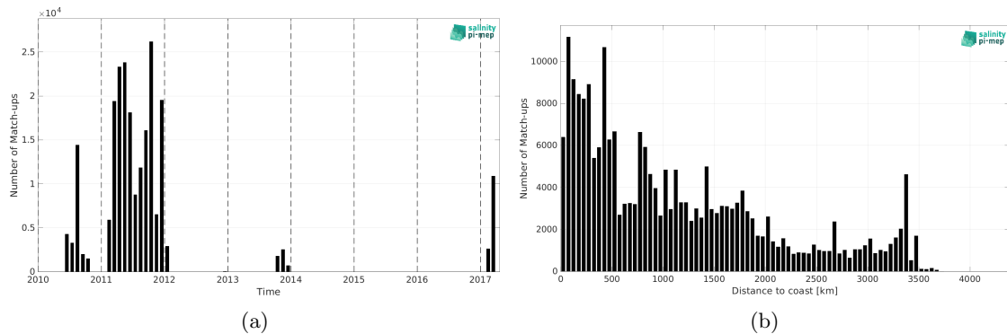
Figure 2: Number of match-ups between TSG (GOSUD-Sailing-ship) and SMOS SSS L3 v335 - Monthly - 25 km (CATDS-CPDC) SSS as a function of time (a) and as function of the distance to coast (b) over the Pacific Ocean Pi-MEP region and for the full satellite product period.
