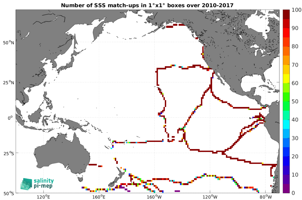
Figure 5: Number of SSS match-ups between TSG (GOSUD-Sailing-ship) SSS and the SMOS SSS L3 v335 - Monthly - 25 km (CATDS-CPDC) SSS product for the Pacific Ocean Pi-MEP region over 1^\circ \times 1^\circ boxes and for the full satellite product period.
