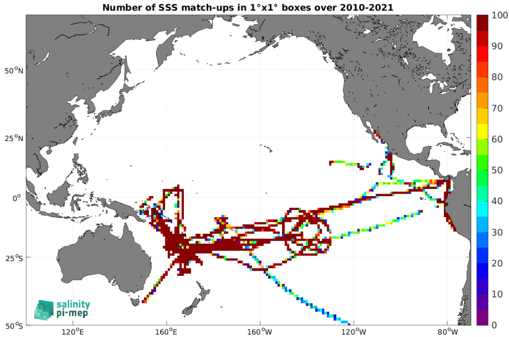
Figure 5: Number of SSS match-ups between TSG (GOSUD-Research-vessel) SSS and the SMOS SSS L3 v335 - Monthly - 25 km (CATDS-CPDC) SSS product for the Pacific Ocean Pi-MEP region over 1^\circ \times 1^\circ boxes and for the full satellite product period.
