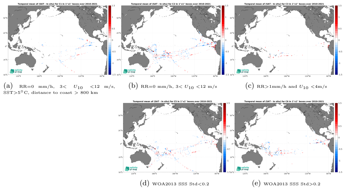
Figure 14: Temporal mean gridded over spatial boxes of size 1^\circ \times 1^\circ of \Delta SSS (SMOS SSS L3 v335 - Monthly - 25 km (CATDS-CPDC) - TSG (GOSUD-Research-vessel)) for 5 different subdatasets corresponding to: RR=0 mm/h, 3 < U_{10} < 12 m/s, SST > 5^\circ\text{C} , distance to coast > 800 km (a), RR=0 mm/h, 3 < U_{10} < 12 m/s (b), RR > 1 mm/h and U_{10} < 4 m/s (c), WOA2013 SSS Std < 0.2 (d), WOA2013 SSS Std > 0.2 (e).
