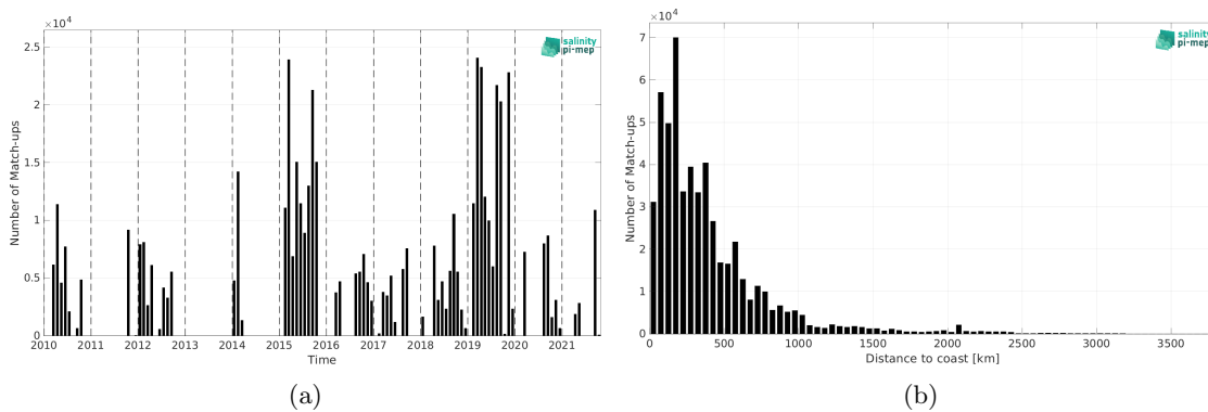
Figure 2: Number of match-ups between TSG (GOSUD-Research-vessel) and SMOS SSS L3 v335 - Monthly - 25 km (CATDS-CPDC) SSS as a function of time (a) and as function of the distance to coast (b) over the Pacific Ocean Pi-MEP region and for the full satellite product period.
