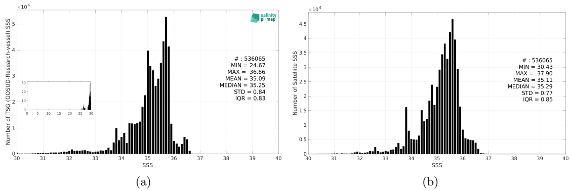
Figure 3: Histograms of SSS from TSG (GOSUD-Research-vessel) (a) and SMOS SSS L3 v335 - Monthly - 25 km (CATDS-CPDC) (b) considering all match-up pairs per bins of 0.1 over the Pacific Ocean Pi-MEP region and for the full satellite product period.
