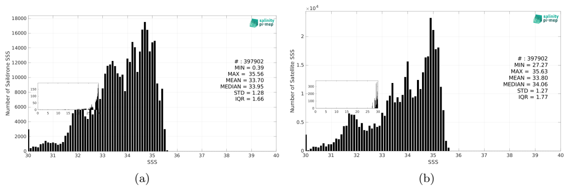
Figure 3: Histograms of SSS from Saildrone (a) and SMOS SSS L3 v335 - Monthly - 25 km (CATDS-CPDC) (b) considering all match-up pairs per bins of 0.1 over the Pacific Ocean Pi-MEP region and for the full satellite product period.
