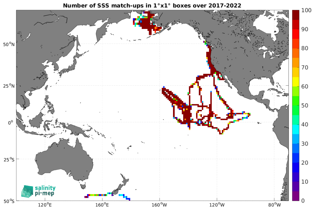
Figure 5: Number of SSS match-ups between Saildrone SSS and the SMOS SSS L3 v335 - Monthly - 25 km (CATDS-CPDC) SSS product for the Pacific Ocean Pi-MEP region over 1^\circ \times 1^\circ boxes and for the full satellite life period.
