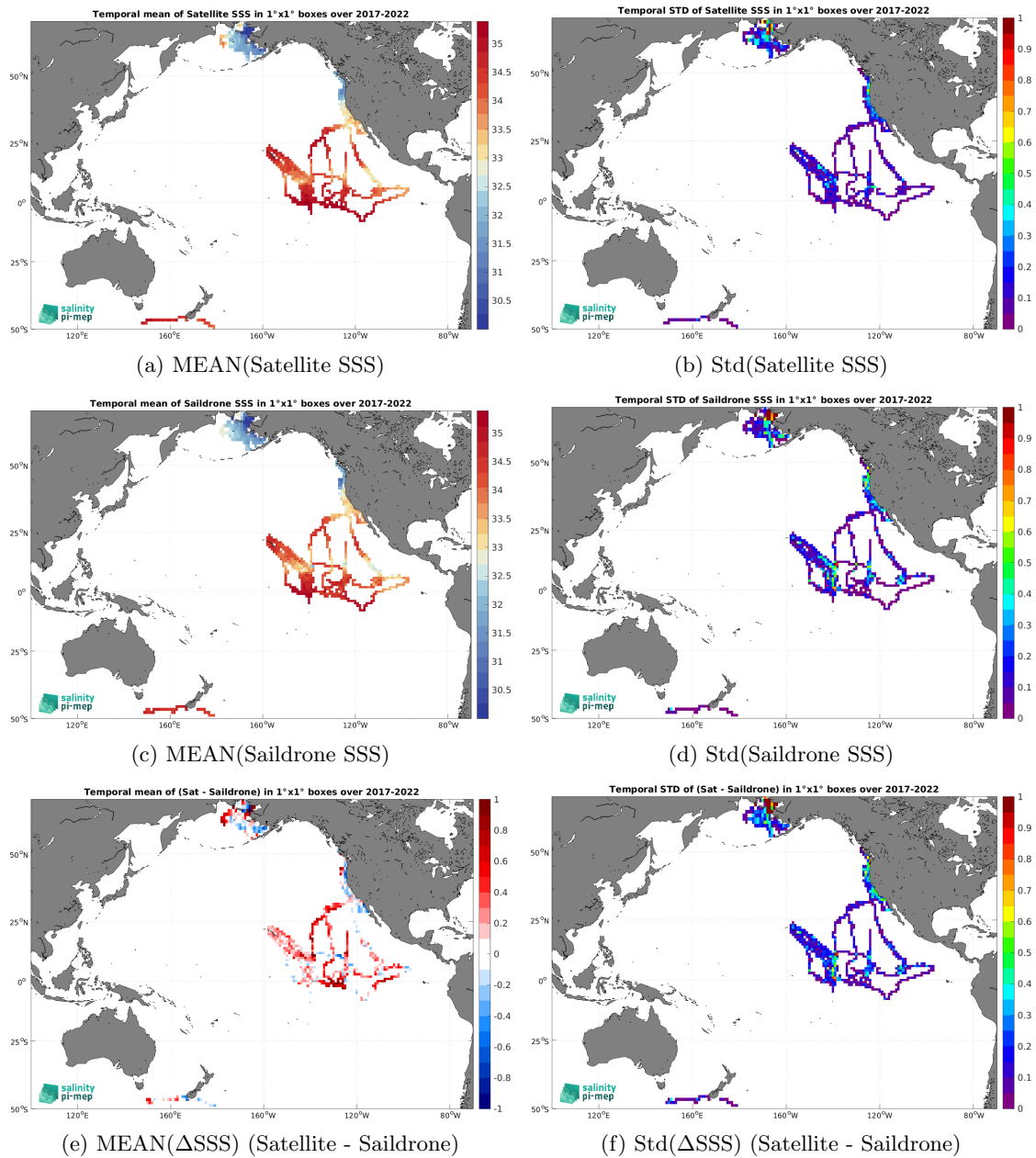
Figure 7: Temporal mean (left) and Std (right) of SSS from SMOS SSS L3 v335 - Monthly - 25 km (CATDS-CPDC) (top), Saildrone (middle), and of \Delta SSS (Satellite - Saildrone). Only match-up pairs are used to generate these maps.
