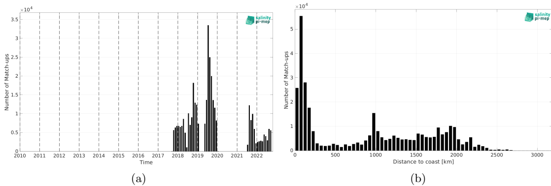
Figure 2: Number of match-ups between Saildrone and SMOS SSS L3 v335 - Monthly - 25 km (CATDS-CPDC) SSS as a function of time (a) and as function of the distance to coast (b) over the Pacific Ocean Pi-MEP region and for the full satellite product period.
