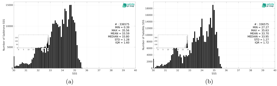
Figure 3: Histograms of SSS from Saildrone (a) and SMOS SSS L3 v335 - Monthly - 25 km (CATDS-CPDC) (b) considering all match-up pairs per bins of 0.1 over the Pacific Ocean Pi-MEP region and for the full satellite product period.
