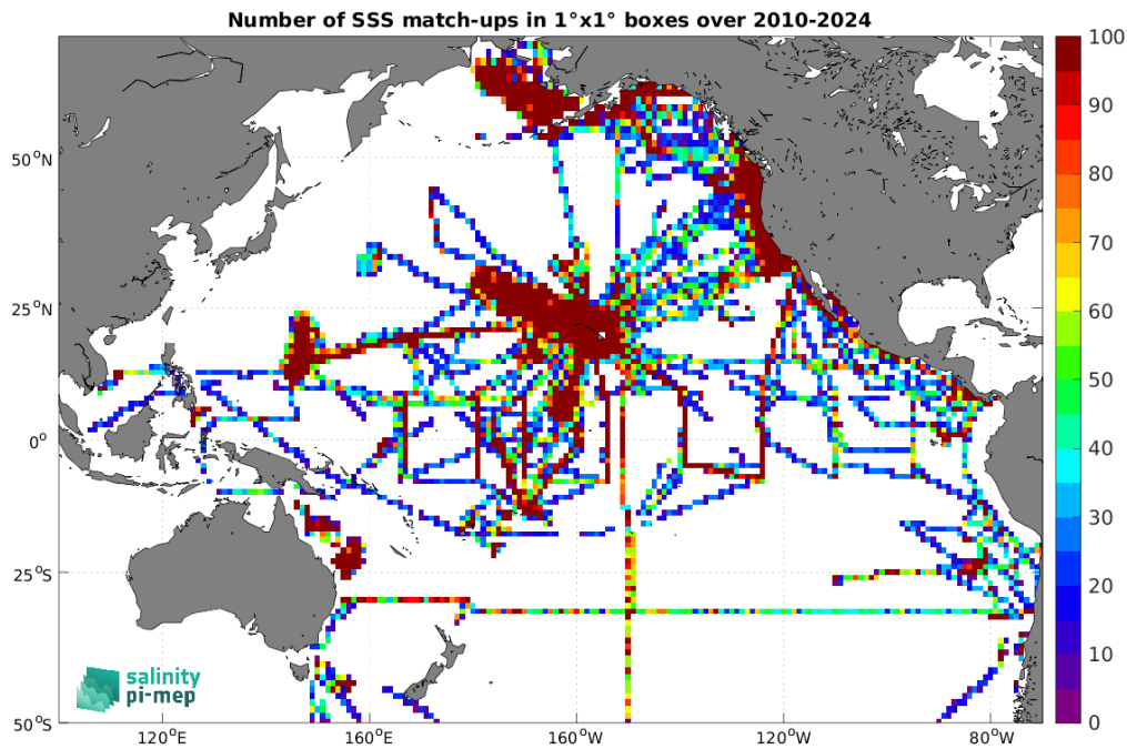
Figure 5: Number of SSS match-ups between TSG (SAMOS) SSS and the SMOS SSS L3 v335 - 10 Days - 25 km (CATDS-CPDC) SSS product for the Pacific Ocean Pi-MEP region over 1^\circ \times 1^\circ boxes and for the full satellite product period.
