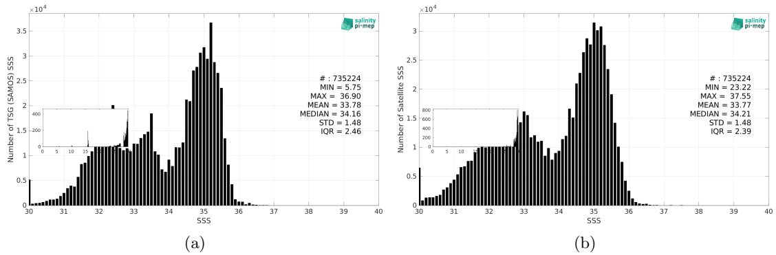
Figure 3: Histograms of SSS from TSG (SAMOS) (a) and SMOS SSS L3 v335 - 10 Days - 25 km (CATDS-CPDC) (b) considering all match-up pairs per bins of 0.1 over the Pacific Ocean Pi-MEP region and for the full satellite product period.
