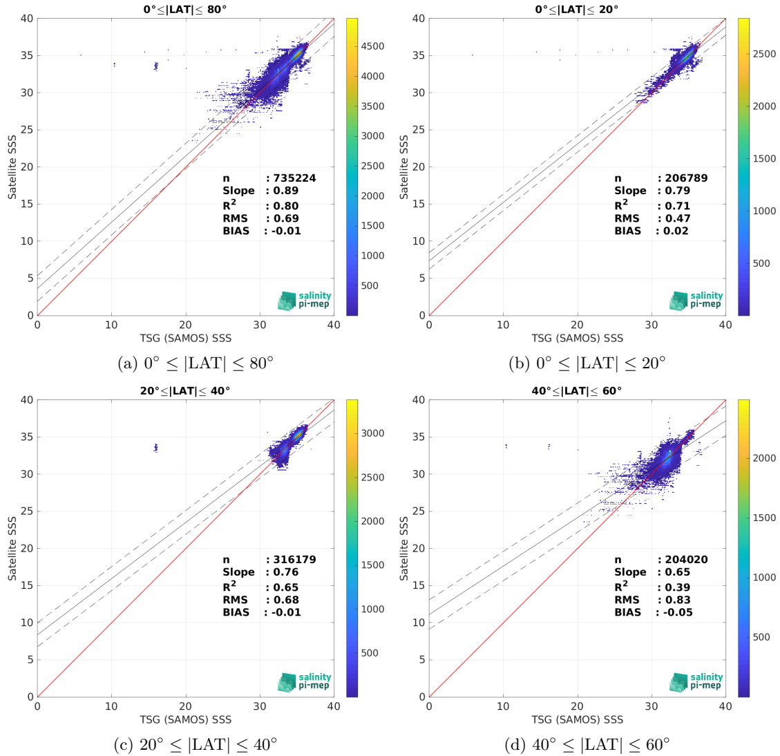
Figure 10: Contour maps of the concentration of SMOS SSS L3 v335 - 10 Days - 25 km (CATDS-CPDC) SSS (y-axis) versus TSG (SAMOS) SSS (x-axis) at match-up pairs for different latitude bands. For each plot, the red line shows x=y . The black thin and dashed lines indicate a linear fit through the data cloud and the \pm 95\% confidence levels, respectively. The number match-up pairs n , the slope and R^2 coefficient of the linear fit, the root mean square (RMS) and the mean bias between satellite and in situ data are indicated for each latitude band in each plots.
