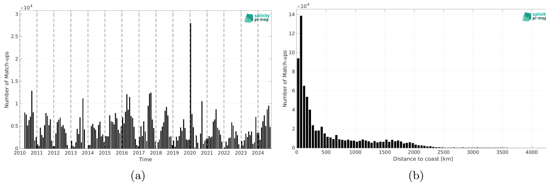
Figure 2: Number of match-ups between TSG (SAMOS) and SMOS SSS L3 v335 - 10 Days - 25 km (CATDS-CPDC) SSS as a function of time (a) and as function of the distance to coast (b) over the Pacific Ocean Pi-MEP region and for the full satellite product period.
