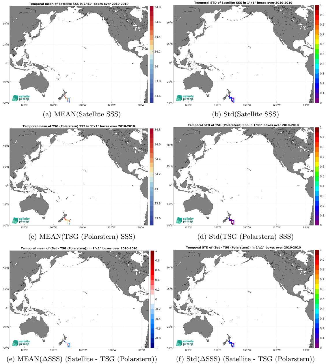
Figure 7: Temporal mean (left) and Std (right) of SSS from SMOS SSS L3 v335 - 10 Days - 25 km (CATDS-CPDC) (top), TSG (Polarstern) (middle), and of \Delta SSS (Satellite - TSG (Polarstern)). Only match-up pairs are used to generate these maps.
