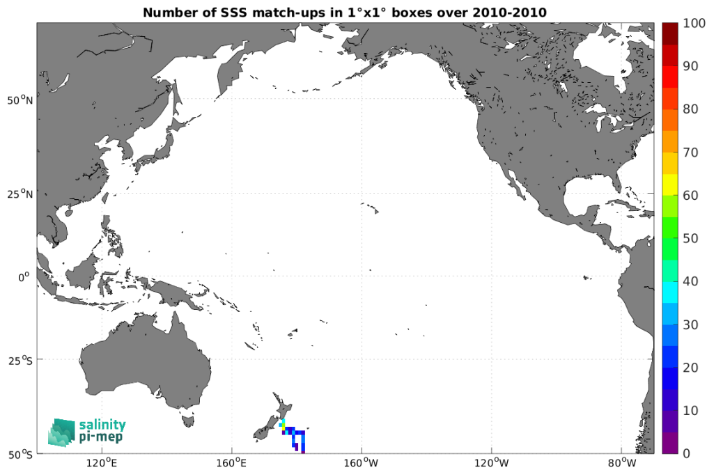
Figure 5: Number of SSS match-ups between TSG (Polarstern) SSS and the SMOS SSS L3 v335 - 10 Days - 25 km (CATDS-CPDC) SSS product for the Pacific Ocean Pi-MEP region over 1^\circ \times 1^\circ boxes and for the full satellite product period.
