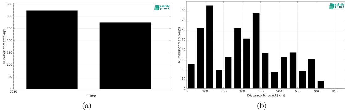
Figure 2: Number of match-ups between TSG (Polarstern) and SMOS SSS L3 v335 - 10 Days - 25 km (CATDS-CPDC) SSS as a function of time (a) and as function of the distance to coast (b) over the Pacific Ocean Pi-MEP region and for the full satellite product period.
