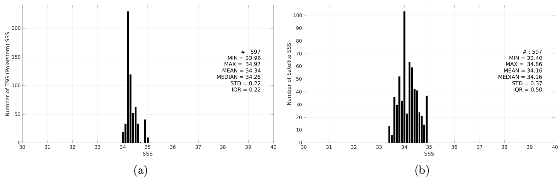
Figure 3: Histograms of SSS from TSG (Polarstern) (a) and SMOS SSS L3 v335 - 10 Days - 25 km (CATDS-CPDC) (b) considering all match-up pairs per bins of 0.1 over the Pacific Ocean Pi-MEP region and for the full satellite product period.
