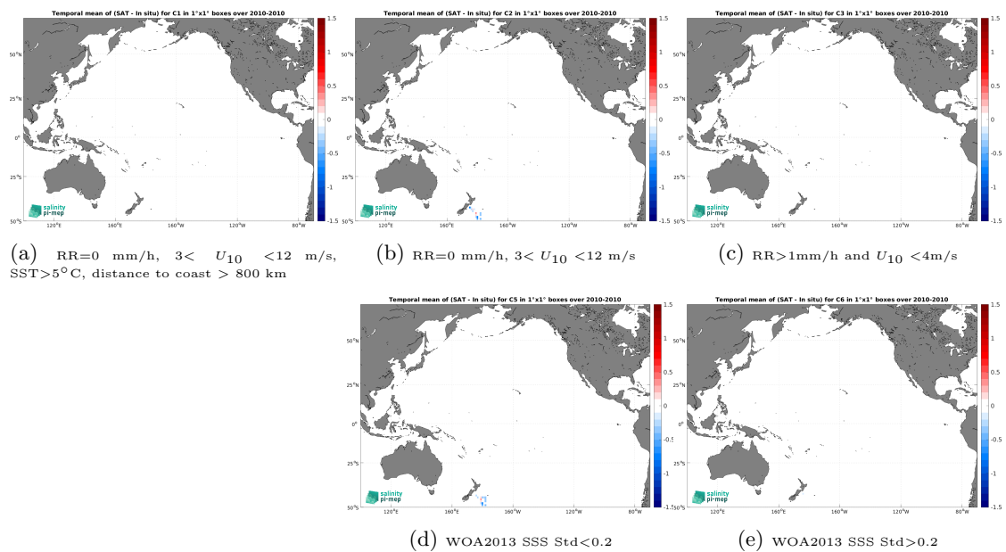
Figure 14: Temporal mean gridded over spatial boxes of size 1^\circ \times 1^\circ of \Delta\text{SSS} (SMOS SSS L3 v335 - 10 Days - 25 km (CATDS-CPDC) - TSG (Polarstern)) for 5 different subdatasets corresponding to:RR=0 mm/h, 3 < U_{10} < 12 m/s, SST > 5^\circ\text{C} , distance to coast > 800 km (a), RR=0 mm/h, 3 < U_{10} < 12 m/s (b), RR > 1 mm/h and U_{10} < 4 m/s (c), WOA2013 SSS Std < 0.2 (d), WOA2013 SSS Std > 0.2 (e).
