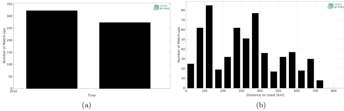
Figure 1: Number of match-ups between TSG (Polarstern) and SMOS SSS L3 v335 - 10 Days - 25 km (CATDS-CPDC) SSS as a function of time (a) and as function of the distance to coast (b) over the Pacific Ocean Pi-MEP region and for the full satellite product period.
