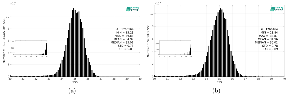
Figure 3: Histograms of SSS from TSG (LEGOS-DM) (a) and SMOS SSS L3 v335 - 10 Days - 25 km (CATDS-CPDC) (b) considering all match-up pairs per bins of 0.1 over the Pacific Ocean Pi-MEP region and for the full satellite product period.
