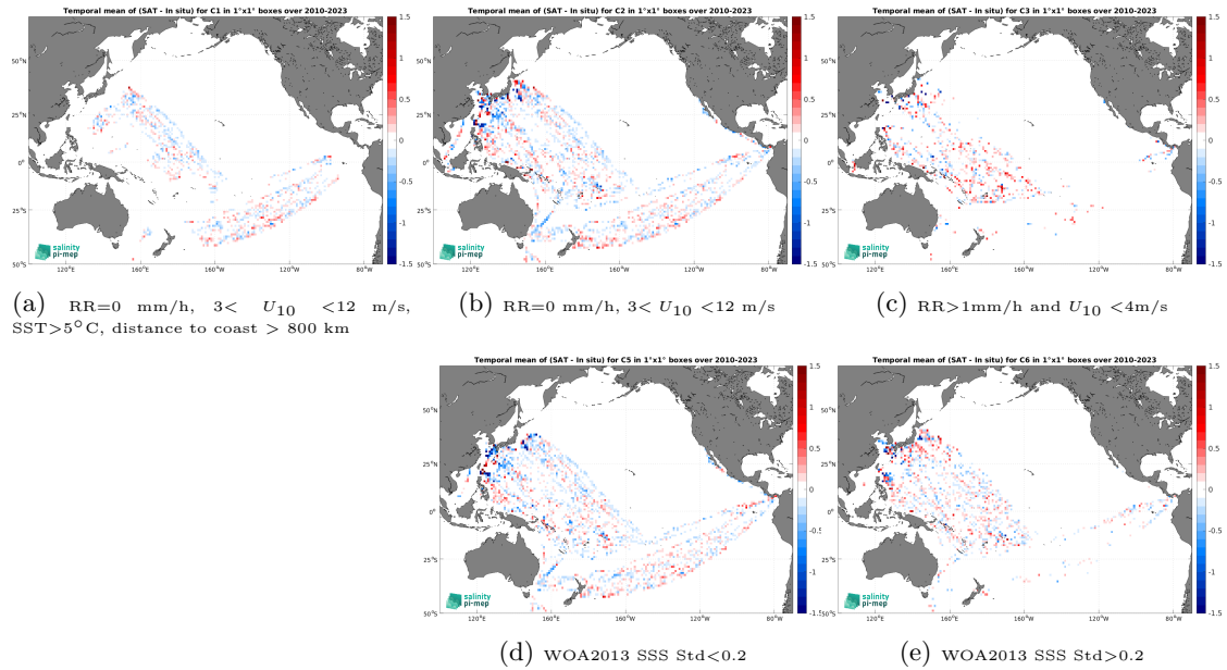
Figure 14: Temporal mean gridded over spatial boxes of size 1^\circ \times 1^\circ of \Delta\text{SSS} (SMOS SSS L3 v335 - 10 Days - 25 km (CATDS-CPDC) - TSG (LEGOS-DM)) for 5 different subdatasets corresponding to:RR=0 mm/h, 3 < U_{10} < 12 m/s, SST >5^\circ\text{C} , distance to coast > 800 km (a), RR=0 mm/h, 3 < U_{10} < 12 m/s (b), RR >1 mm/h and U_{10} < 4 m/s (c), WOA2013 SSS Std <0.2 (d), WOA2013 SSS Std >0.2 (e).
