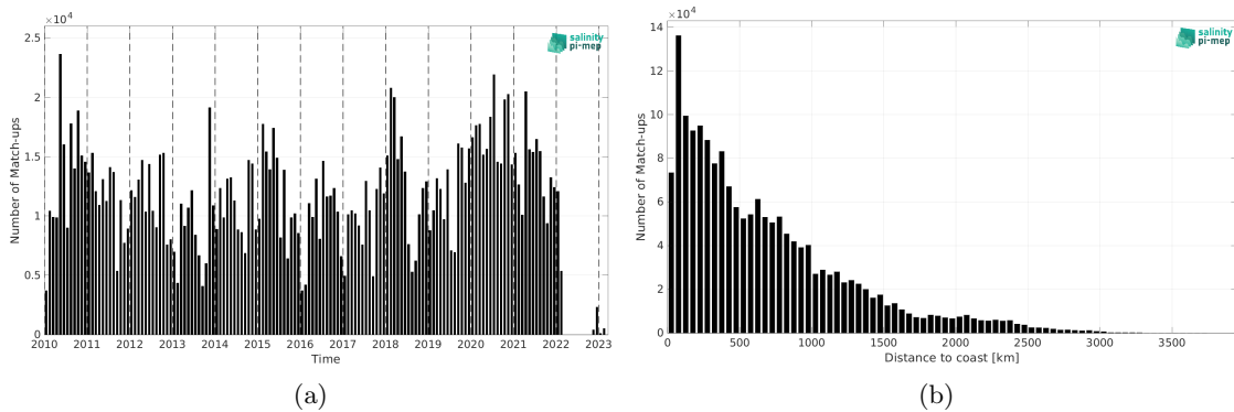
Figure 2: Number of match-ups between TSG (LEGOS-DM) and SMOS SSS L3 v335 - 10 Days - 25 km (CATDS-CPDC) SSS as a function of time (a) and as function of the distance to coast (b) over the Pacific Ocean Pi-MEP region and for the full satellite product period.
