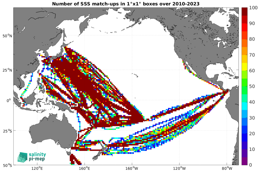
Figure 5: Number of SSS match-ups between TSG (LEGOS-DM) SSS and the SMOS SSS L3 v335 - 10 Days - 25 km (CATDS-CPDC) SSS product for the Pacific Ocean Pi-MEP region over 1^\circ \times 1^\circ boxes and for the full satellite product period.
