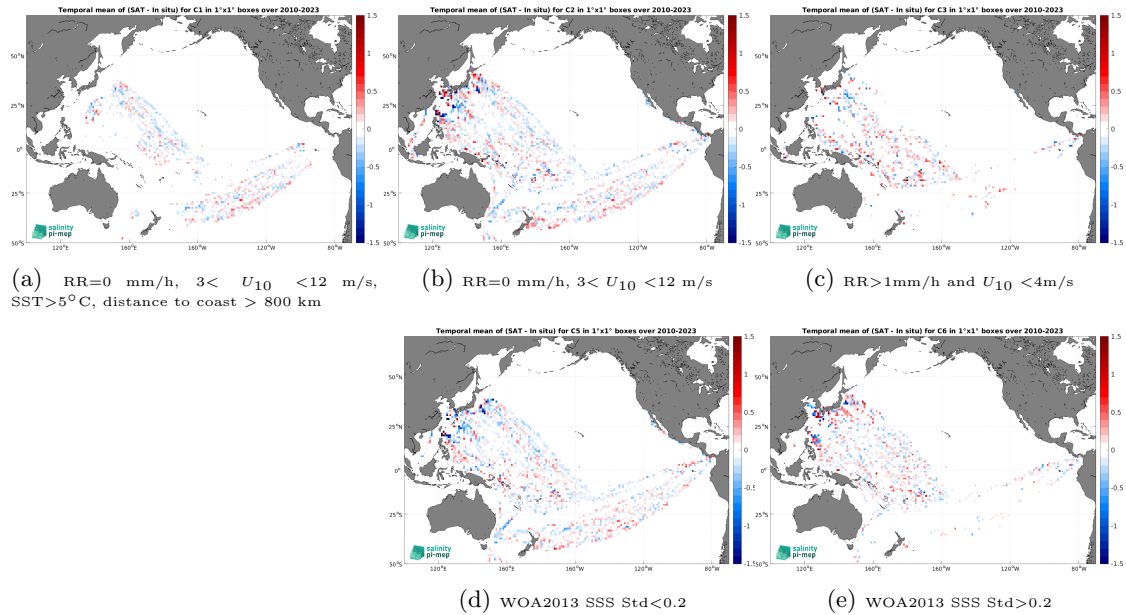
Figure 12: Temporal mean gridded over spatial boxes of size 1^\circ \times 1^\circ of \Delta\text{SSS} (SMOS SSS L3 v335 - 10 Days - 25 km (CATDS-CPDC) - TSG (LEGOS-DM)) for 5 different subdatasets corresponding to:RR=0 mm/h, 3 < U_{10} < 12 m/s, SST >5^\circ\text{C} , distance to coast > 800 km (a), RR=0 mm/h, 3 < U_{10} < 12 m/s (b), RR >1 mm/h and U_{10} < 4 m/s (c), WOA2013 SSS Std <0.2 (d), WOA2013 SSS Std >0.2 (e).
