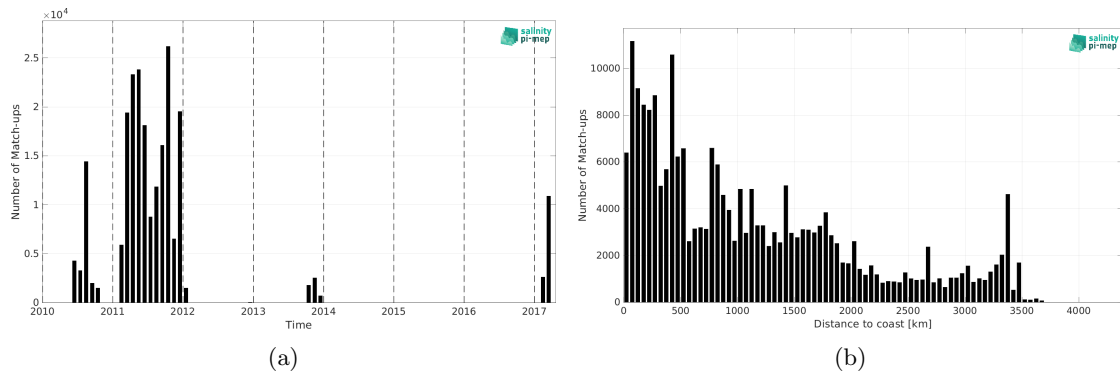
Figure 2: Number of match-ups between TSG (GOSUD-Sailing-ship) and SMOS SSS L3 v335 - 10 Days - 25 km (CATDS-CPDC) SSS as a function of time (a) and as function of the distance to coast (b) over the Pacific Ocean Pi-MEP region and for the full satellite product period.
