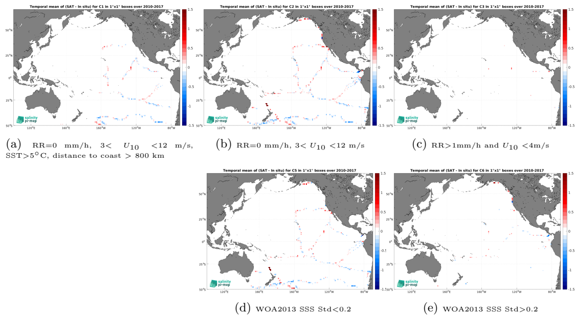
Figure 14: Temporal mean gridded over spatial boxes of size 1^\circ \times 1^\circ of \Delta SSS (SMOS SSS L3 v335 - 10 Days - 25 km (CATDS-CPDC) - TSG (GOSUD-Sailing-ship)) for 5 different subdatasets corresponding to:RR=0 mm/h, 3 < U_{10} < 12 m/s, SST >5^\circ\text{C} , distance to coast > 800 km (a), RR=0 mm/h, 3 < U_{10} < 12 m/s (b), RR >1 mm/h and U_{10} < 4 m/s (c), WOA2013 SSS Std <0.2 (d), WOA2013 SSS Std >0.2 (e).
