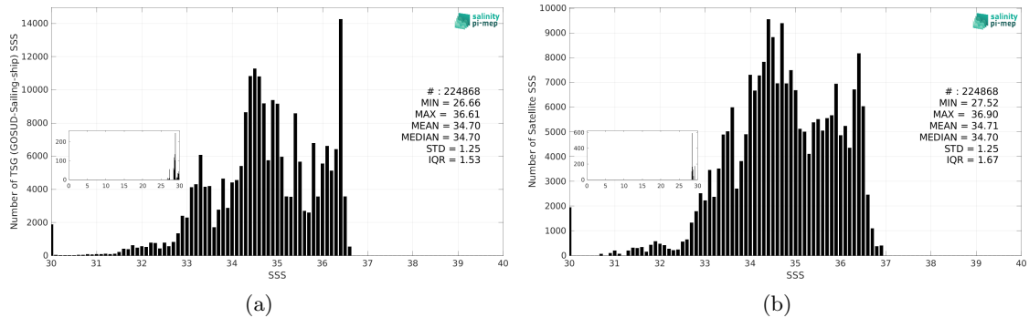
Figure 3: Histograms of SSS from TSG (GOSUD-Sailing-ship) (a) and SMOS SSS L3 v335 - 10 Days - 25 km (CATDS-CPDC) (b) considering all match-up pairs per bins of 0.1 over the Pacific Ocean Pi-MEP region and for the full satellite product period.
