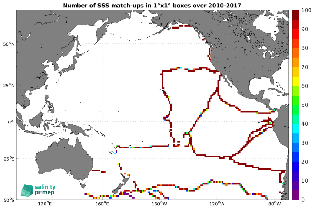
Figure 5: Number of SSS match-ups between TSG (GOSUD-Sailing-ship) SSS and the SMOS SSS L3 v335 - 10 Days - 25 km (CATDS-CPDC) SSS product for the Pacific Ocean Pi-MEP region over 1^\circ \times 1^\circ boxes and for the full satellite product period.
