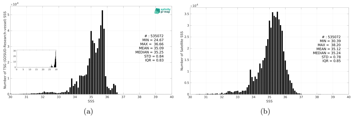
Figure 3: Histograms of SSS from TSG (GOSUD-Research-vessel) (a) and SMOS SSS L3 v335 - 10 Days - 25 km (CATDS-CPDC) (b) considering all match-up pairs per bins of 0.1 over the Pacific Ocean Pi-MEP region and for the full satellite product period.
