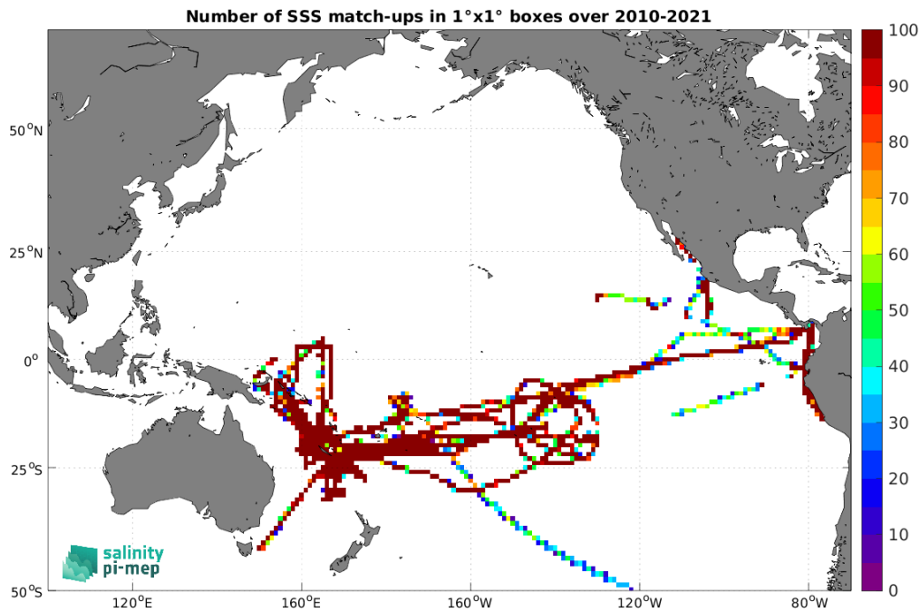
Figure 5: Number of SSS match-ups between TSG (GOSUD-Research-vessel) SSS and the SMOS SSS L3 v335 - 10 Days - 25 km (CATDS-CPDC) SSS product for the Pacific Ocean Pi-MEP region over 1^\circ \times 1^\circ boxes and for the full satellite product period.
