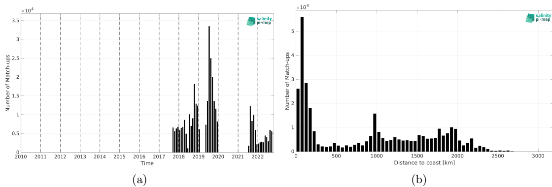
Figure 2: Number of match-ups between Saildrone and SMOS SSS L3 v335 - 10 Days - 25 km (CATDS-CPDC) SSS as a function of time (a) and as function of the distance to coast (b) over the Pacific Ocean Pi-MEP region and for the full satellite product period.
