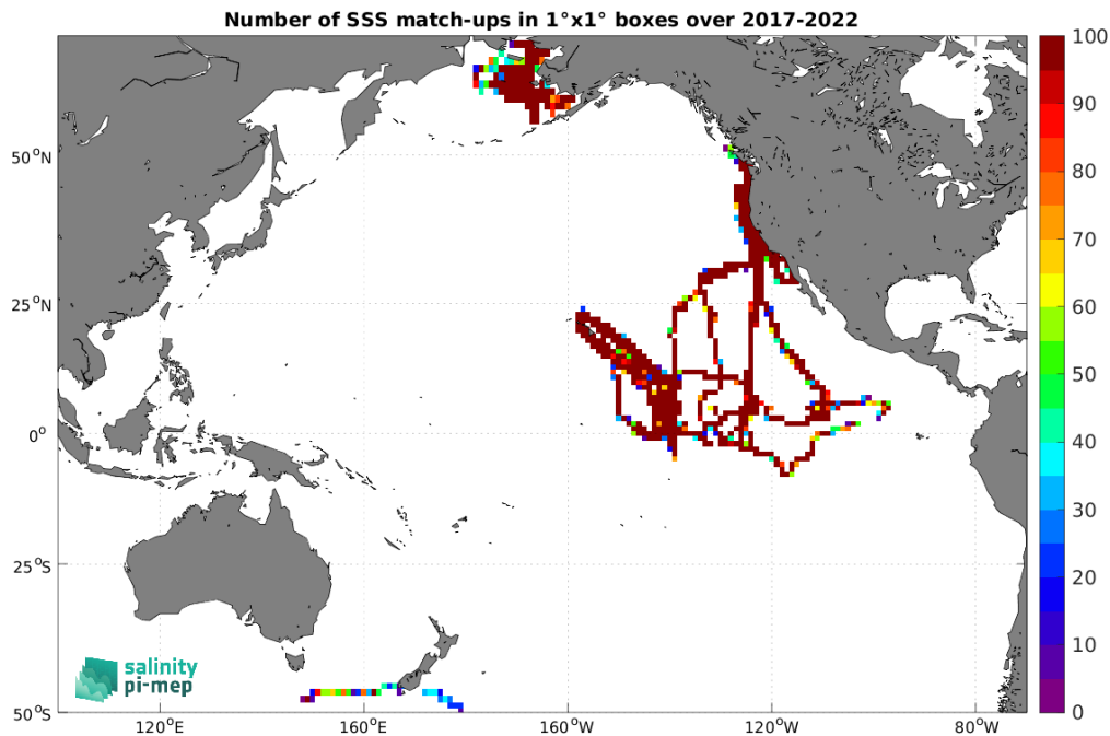
Figure 5: Number of SSS match-ups between Saildrone SSS and the SMOS SSS L3 v335 - 10 Days - 25 km (CATDS-CPDC) SSS product for the Pacific Ocean Pi-MEP region over 1^\circ \times 1^\circ boxes and for the full satellite product period.
