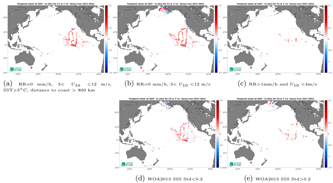
Figure 14: Temporal mean gridded over spatial boxes of size 1^\circ \times 1^\circ of \Delta SSS (SMOS SSS L3 v335 - 10 Days - 25 km (CATDS-CPDC) - Saildrone) for 5 different subdatasets corresponding to:RR=0 mm/h, 3 < U_{10} < 12 m/s, SST >5^\circ\text{C} , distance to coast > 800 km (a), RR=0 mm/h, 3 < U_{10} < 12 m/s (b), RR >1 mm/h and U_{10} < 4 m/s (c), WOA2013 SSS Std <0.2 (d), WOA2013 SSS Std >0.2 (e).
