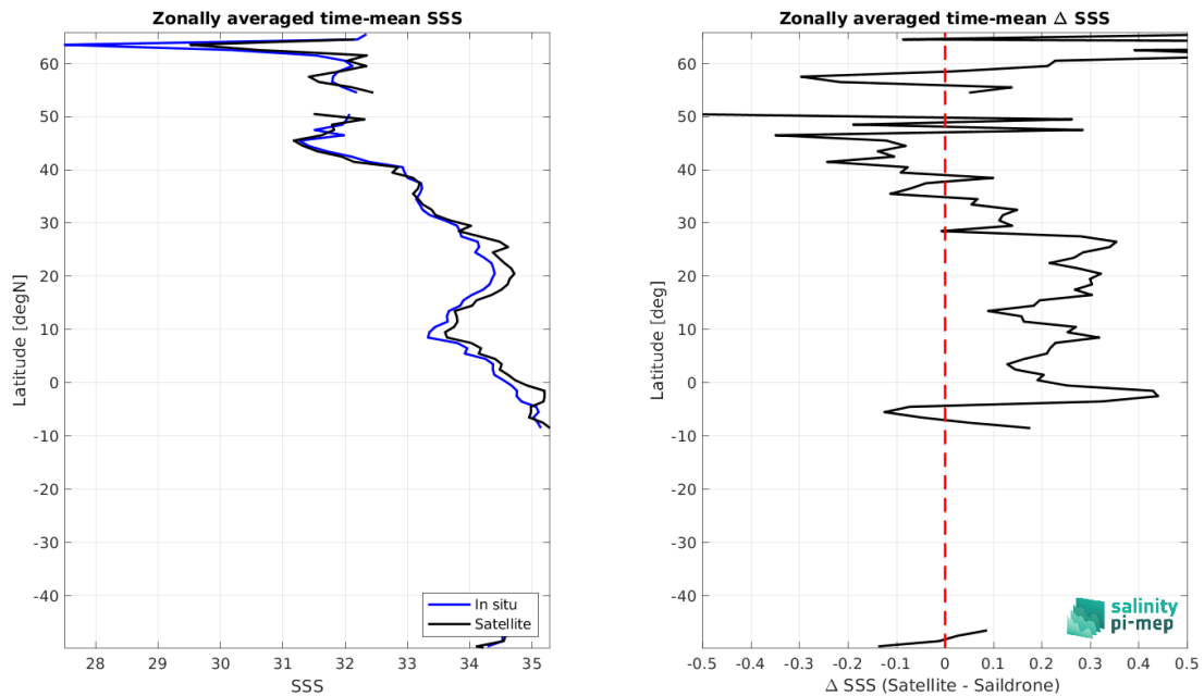
Figure 9: Left panel: Zonal mean SSS from SMOS SSS L3 v335 - 10 Days - 25 km (CATDS-CPDC) satellite product (black) and from Saldrone (blue). Right panel: Zonal mean of \Delta SSS (Satellite - Saldrone) for all the collected Pi-MEP match-up pairs estimated over the full satellite product period.
