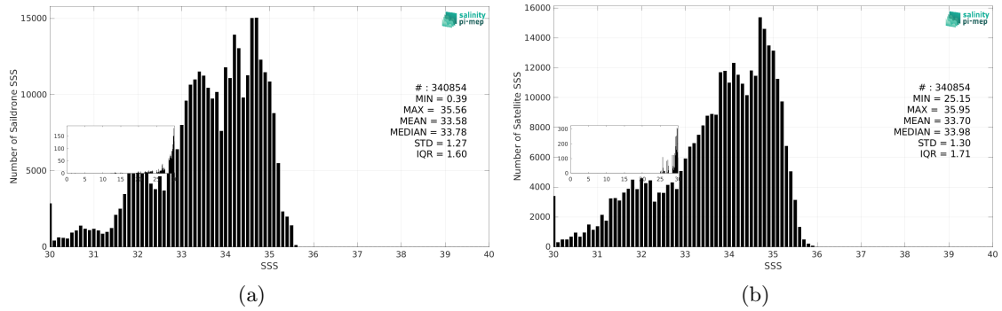
Figure 3: Histograms of SSS from Saildrone (a) and SMOS SSS L3 v335 - 10 Days - 25 km (CATDS-CPDC) (b) considering all match-up pairs per bins of 0.1 over the Pacific Ocean Pi-MEP region and for the full satellite product period.
