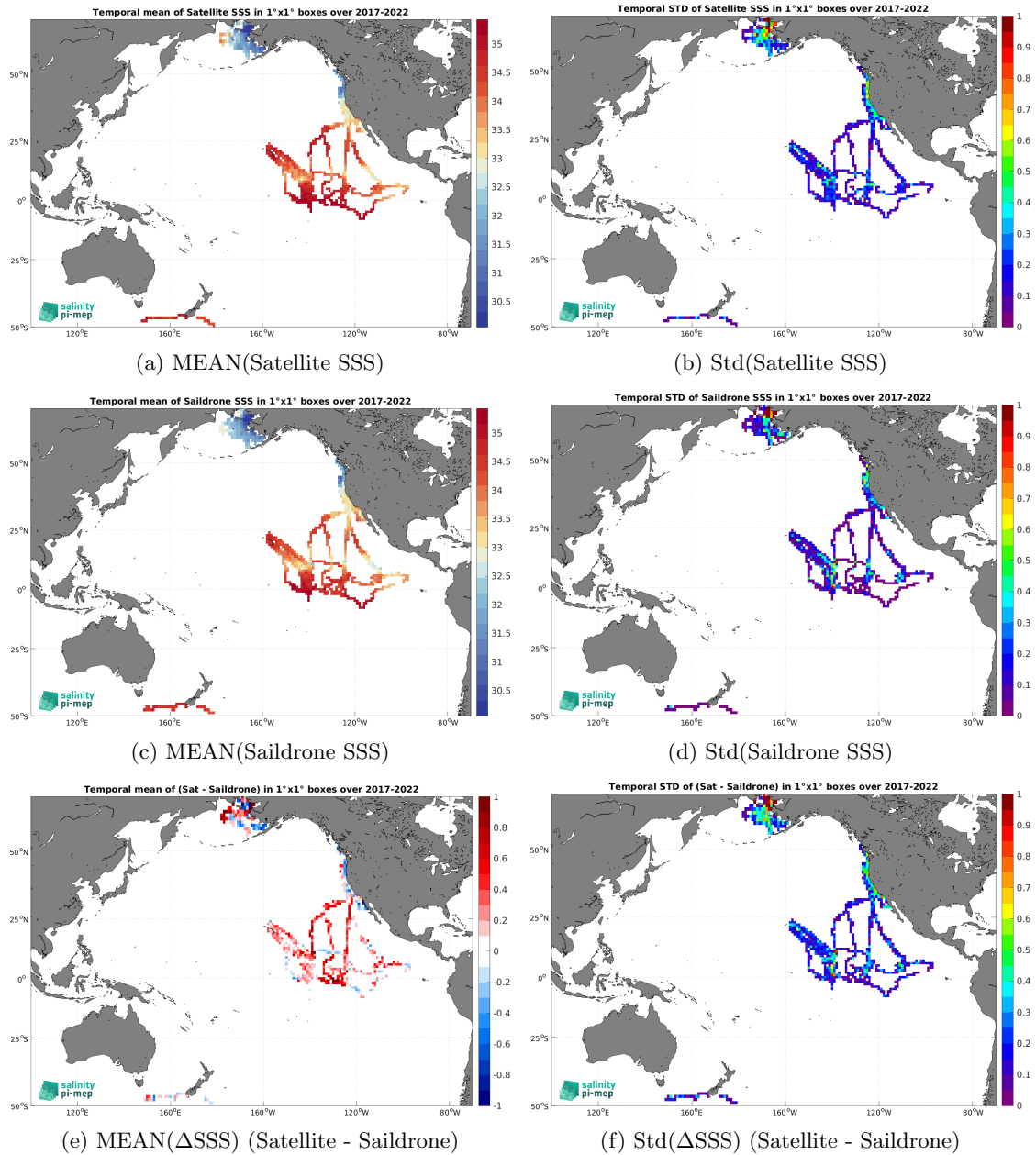
Figure 7: Temporal mean (left) and Std (right) of SSS from SMOS SSS L3 v335 - 10 Days - 25 km (CATDS-CPDC) (top), Saildrone (middle), and of \Delta SSS (Satellite - Saildrone). Only match-up pairs are used to generate these maps.
