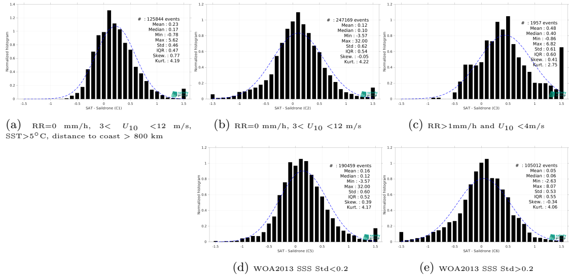
Figure 15: Normalized histogram of \Delta SSS (SMOS SSS L3 v335 - 10 Days - 25 km (CATDS-CPDC) - Salldrone) for 5 different subdatasets corresponding to: RR=0 mm/h, 3 < U_{10} < 12 m/s, SST>5°C, distance to coast > 800 km (a), RR=0 mm/h, 3 < U_{10} < 12 m/s (b), RR>1mm/h and U_{10} < 4 m/s (c), WOA2013 SSS Std<0.2 (d), WOA2013 SSS Std>0.2 (e).
