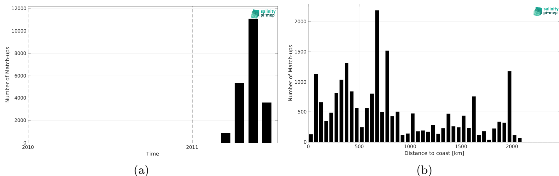
Figure 2: Number of match-ups between TSG (CSIC-UTM) and SMOS SSS L2Q v333 - 0.25 Deg (CATDS-CPDC) SSS as a function of time (a) and as function of the distance to coast (b) over the Pacific Ocean Pi-MEP region and for the full satellite product period.
