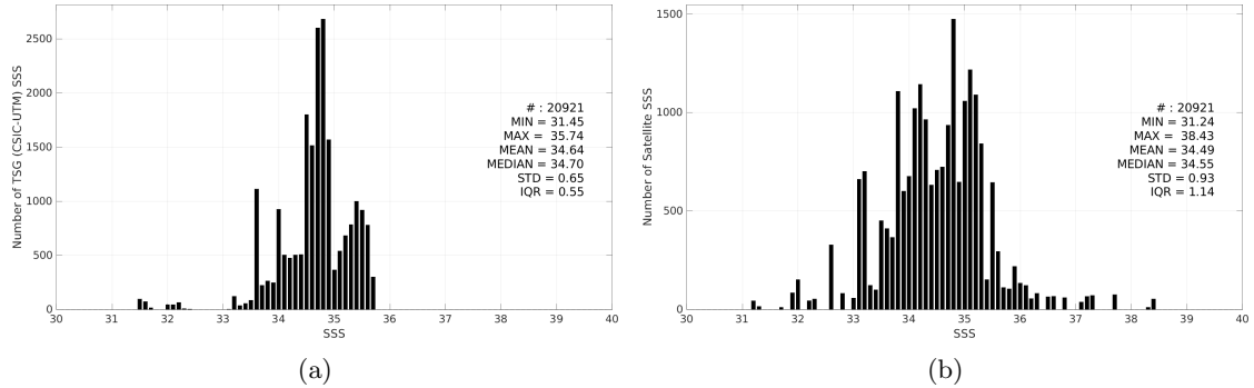
Figure 3: Histograms of SSS from TSG (CSIC-UTM) (a) and SMOS SSS L2Q v333 - 0.25 Deg (CATDS-CPDC) (b) considering all match-up pairs per bins of 0.1 over the Pacific Ocean Pi-MEP region and for the full satellite product period.
