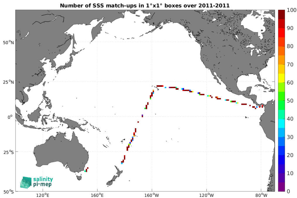
Figure 5: Number of SSS match-ups between TSG (CSIC-UTM) SSS and the SMOS SSS L2Q v333 - 0.25 Deg (CATDS-CPDC) SSS product for the Pacific Ocean Pi-MEP region over 1^\circ \times 1^\circ boxes and for the full satellite product period.
