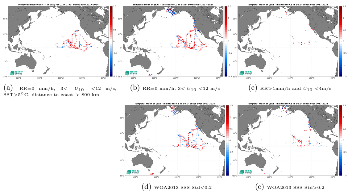
Figure 14: Temporal mean gridded over spatial boxes of size 1^\circ \times 1^\circ of \Delta SSS (SMOS SSS L2Q v333 - 0.25 Deg (CATDS-CPDC) - Saildrone) for 5 different subdatasets corresponding to:RR=0 mm/h, 3 < U_{10} < 12 m/s, SST > 5^\circ\text{C} , distance to coast > 800 km (a), RR=0 mm/h, 3 < U_{10} < 12 m/s (b), RR > 1 mm/h and U_{10} < 4 m/s (c), WOA2013 SSS Std < 0.2 (d), WOA2013 SSS Std > 0.2 (e).
