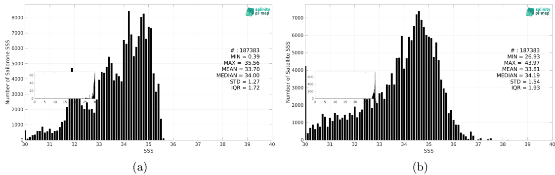
Figure 3: Histograms of SSS from Saildrone (a) and SMOS SSS L2Q v333 - 0.25 Deg (CATDS-CPDC) (b) considering all match-up pairs per bins of 0.1 over the Pacific Ocean Pi-MEP region and for the full satellite product period.
