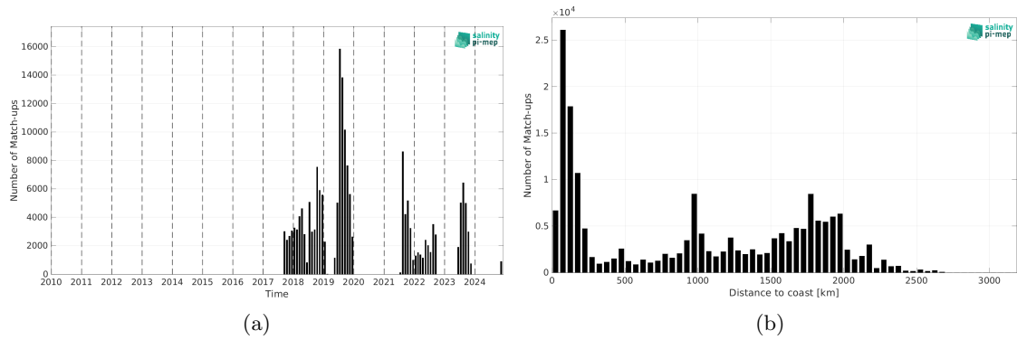
Figure 2: Number of match-ups between Saildrone and SMOS SSS L2Q v333 - 0.25 Deg (CATDS-CPDC) SSS as a function of time (a) and as function of the distance to coast (b) over the Pacific Ocean Pi-MEP region and for the full satellite product period.
