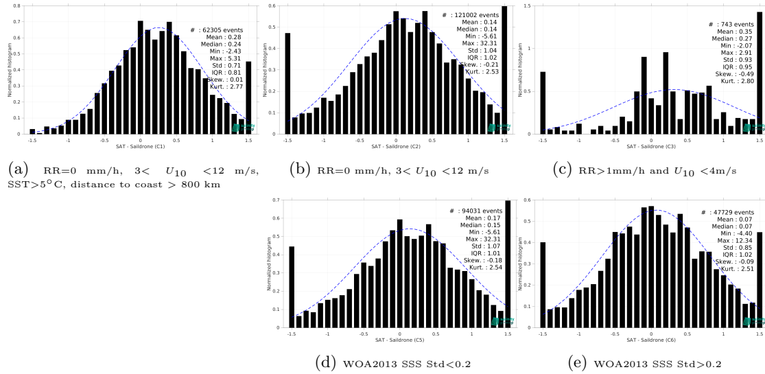
Figure 15: Normalized histogram of \Delta SSS (SMOS SSS L2Q v333 - 0.25 Deg (CATDS-CPDC) - Sairdron) for 5 different subdatasets corresponding to: RR=0 mm/h, 3 < U_{10} < 12 m/s, SST>5°C, distance to coast > 800 km (a), RR=0 mm/h, 3 < U_{10} < 12 m/s (b), RR>1mm/h and U_{10} < 4 m/s (c), WOA2013 SSS Std<0.2 (d), WOA2013 SSS Std>0.2 (e).
