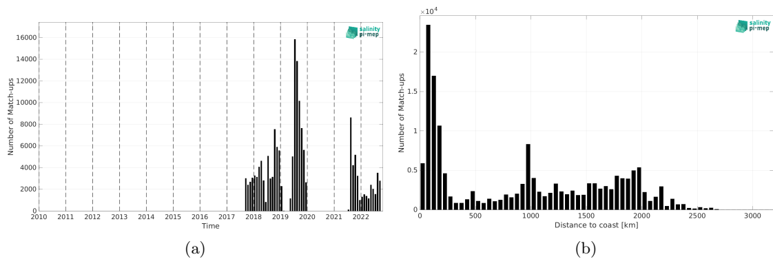
Figure 2: Number of match-ups between Sairdrone and SMOS SSS L2Q v333 - 0.25 Deg (CATDS-CPDC) SSS as a function of time (a) and as function of the distance to coast (b) over the Pacific Ocean Pi-MEP region and for the full satellite product period.
