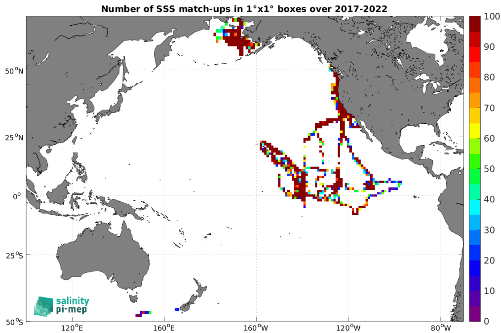
Figure 5: Number of SSS match-ups between Saildrone SSS and the SMOS SSS L2Q v333 - 0.25 Deg (CATDS-CPDC) SSS product for the Pacific Ocean Pi-MEP region over 1^\circ \times 1^\circ boxes and for the full satellite product period.
