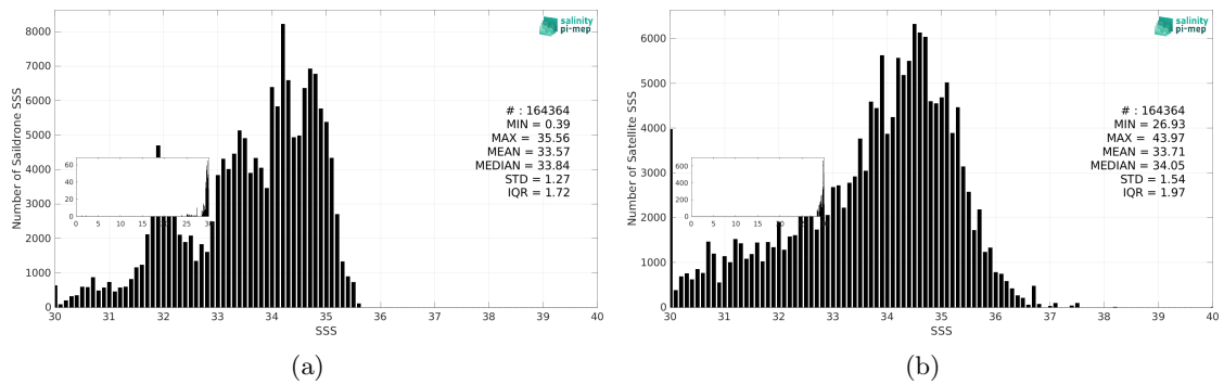
Figure 3: Histograms of SSS from Sairdrone (a) and SMOS SSS L2Q v333 - 0.25 Deg (CATDS-CPDC) (b) considering all match-up pairs per bins of 0.1 over the Pacific Ocean Pi-MEP region and for the full satellite product period.
