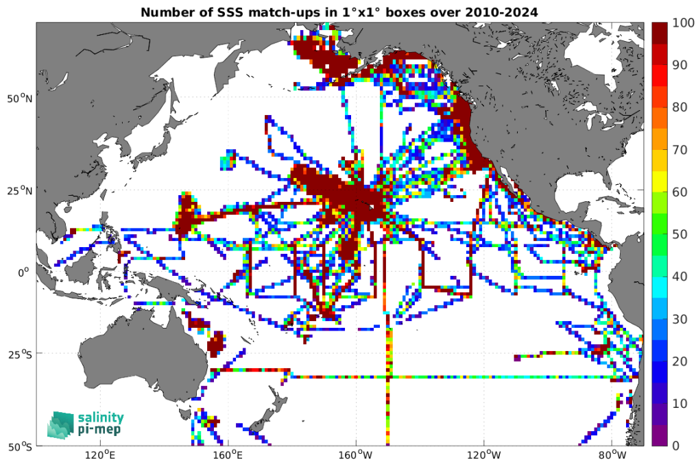
Figure 5: Number of SSS match-ups between TSG (SAMOS) SSS and the SMOS SSS L3 v332 - 9 Days (CATDS-CPDC) SSS product for the Pacific Ocean Pi-MEP region over 1^\circ \times 1^\circ boxes and for the full satellite product period.
