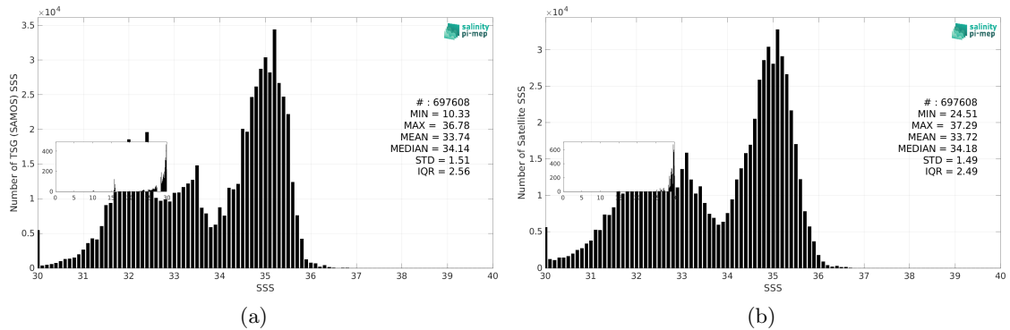
Figure 3: Histograms of SSS from TSG (SAMOS) (a) and SMOS SSS L3 v332 - 9 Days (CATDS-CPDC) (b) considering all match-up pairs per bins of 0.1 over the Pacific Ocean Pi-MEP region and for the full satellite product period.
