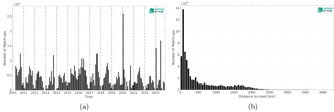
Figure 1: Number of match-ups between TSG (SAMOS) and SMOS SSS L3 v332 - 9 Days (CATDS-CPDC) SSS as a function of time (a) and as function of the distance to coast (b) over the Pacific Ocean Pi-MEP region and for the full satellite product period.
