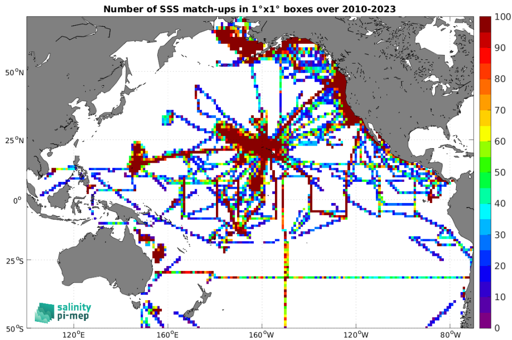
Figure 4: Number of SSS match-ups between TSG (SAMOS) SSS and the SMOS SSS L3 v332 - 9 Days (CATDS-CPDC) SSS product for the Pacific Ocean Pi-MEP region over 1^\circ \times 1^\circ boxes and for the full satellite product period.
