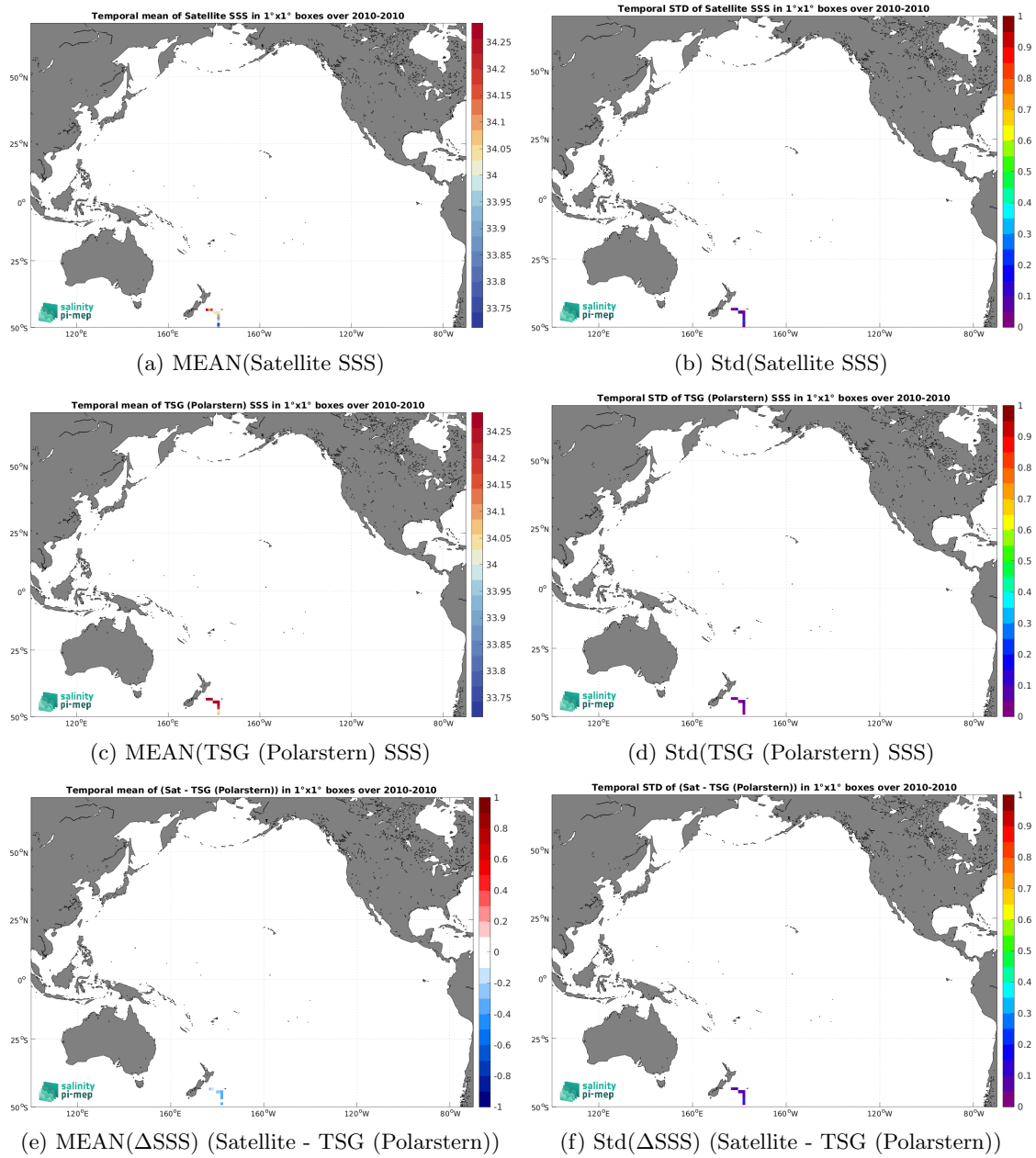
Figure 7: Temporal mean (left) and Std (right) of SSS from SMOS SSS L3 v332 - 9 Days (CATDS-CPDC) (top), TSG (Polarstern) (middle), and of \Delta SSS (Satellite - TSG (Polarstern)). Only match-up pairs are used to generate these maps.
