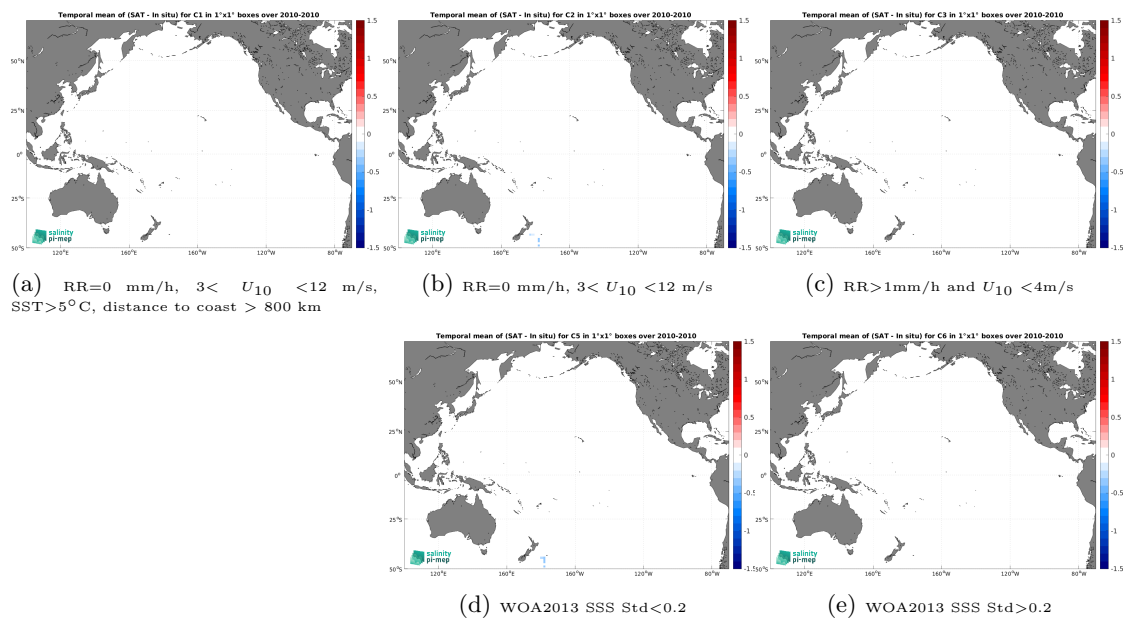
Figure 14: Temporal mean gridded over spatial boxes of size 1^\circ \times 1^\circ of \Delta\text{SSS} (SMOS SSS L3 v332 - 9 Days (CATDS-CPDC) - TSG (Polarstern)) for 5 different subdatasets corresponding to: RR=0 mm/h, 3 < U_{10} < 12 m/s, SST > 5^\circ\text{C} , distance to coast > 800 km (a), RR=0 mm/h, 3 < U_{10} < 12 m/s (b), RR > 1 mm/h and U_{10} < 4 m/s (c), WOA2013 SSS Std < 0.2 (d), WOA2013 SSS Std > 0.2 (e).
