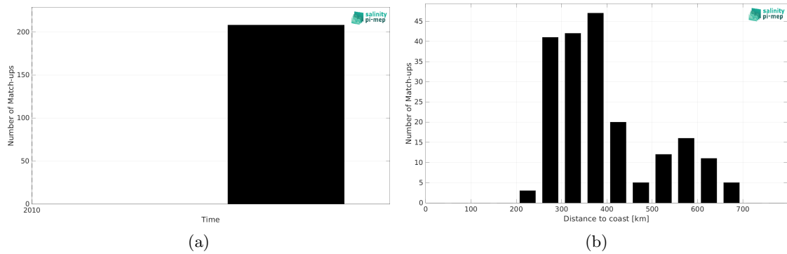
Figure 2: Number of match-ups between TSG (Polarstern) and SMOS SSS L3 v332 - 9 Days (CATDS-CPDC) SSS as a function of time (a) and as function of the distance to coast (b) over the Pacific Ocean Pi-MEP region and for the full satellite product period.
