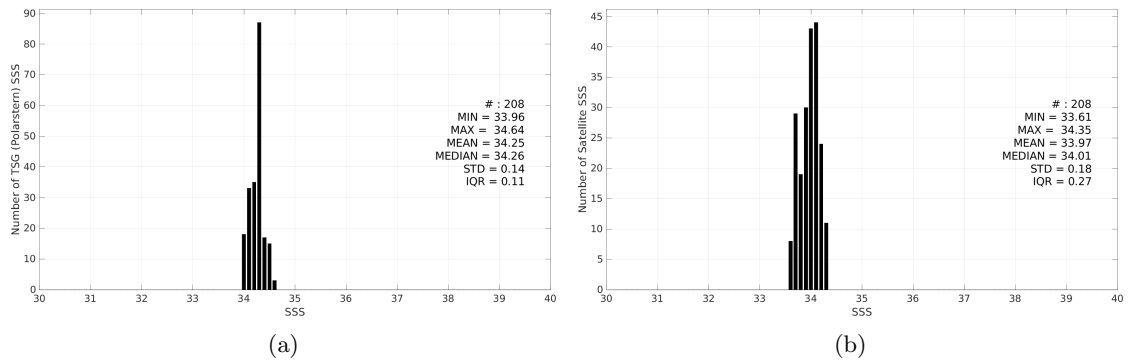
Figure 3: Histograms of SSS from TSG (Polarstern) (a) and SMOS SSS L3 v332 - 9 Days (CATDS-CPDC) (b) considering all match-up pairs per bins of 0.1 over the Pacific Ocean Pi-MEP region and for the full satellite product period.
