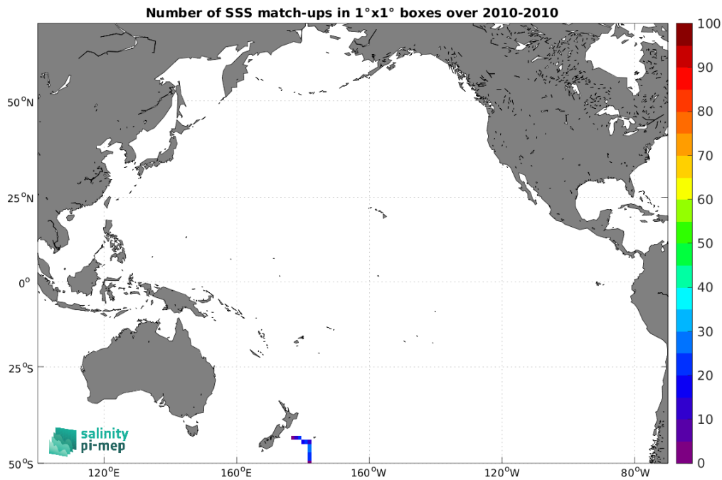
Figure 5: Number of SSS match-ups between TSG (Polarstern) SSS and the SMOS SSS L3 v332 - 9 Days (CATDS-CPDC) SSS product for the Pacific Ocean Pi-MEP region over 1^\circ \times 1^\circ boxes and for the full satellite product period.
