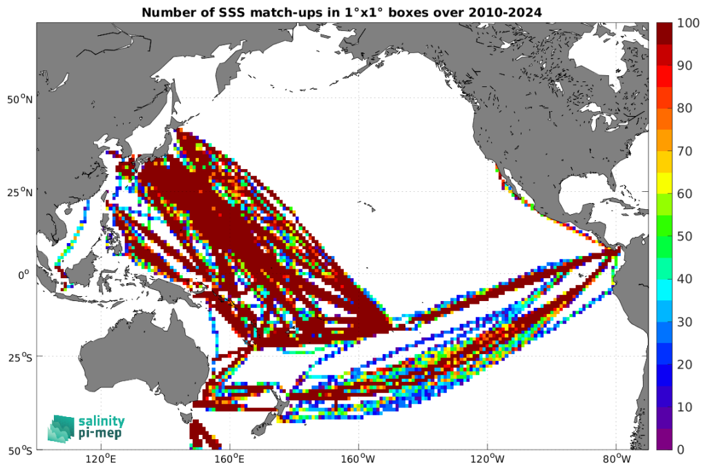
Figure 5: Number of SSS match-ups between TSG (LEGOS-DM) SSS and the SMOS SSS L3 v332 - 9 Days (CATDS-CPDC) SSS product for the Pacific Ocean Pi-MEP region over 1^\circ \times 1^\circ boxes and for the full satellite product period.
