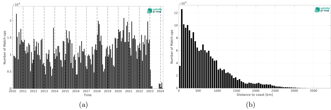
Figure 2: Number of match-ups between TSG (LEGOS-DM) and SMOS SSS L3 v332 - 9 Days (CATDS-CPDC) SSS as a function of time (a) and as function of the distance to coast (b) over the Pacific Ocean Pi-MEP region and for the full satellite product period.
