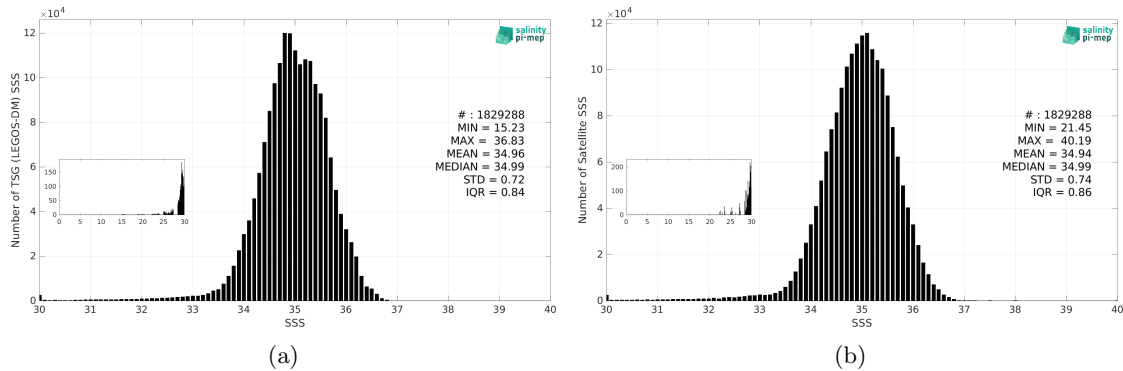
Figure 3: Histograms of SSS from TSG (LEGOS-DM) (a) and SMOS SSS L3 v332 - 9 Days (CATDS-CPDC) (b) considering all match-up pairs per bins of 0.1 over the Pacific Ocean Pi-MEP region and for the full satellite product period.
