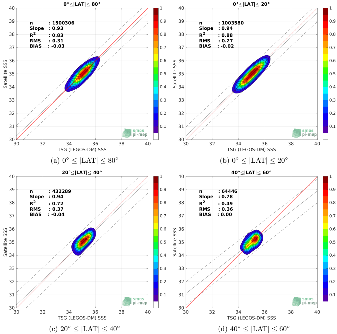
Figure 9: Contour maps of the concentration of SMOS SSS L3 v332 - 9 Days (CATDS-CPDC) SSS (y-axis) versus TSG (LEGOS-DM) SSS (x-axis) at match-up pairs for different latitude bands. For each plot, the red line shows x=y . The black thin and dashed lines indicate a linear fit through the data cloud and the \pm 95\% confidence levels, respectively. The number match-up pairs n , the slope and R^2 coefficient of the linear fit, the root mean square (RMS) and the mean bias between satellite and in situ data are indicated for each latitude band in each plots.
