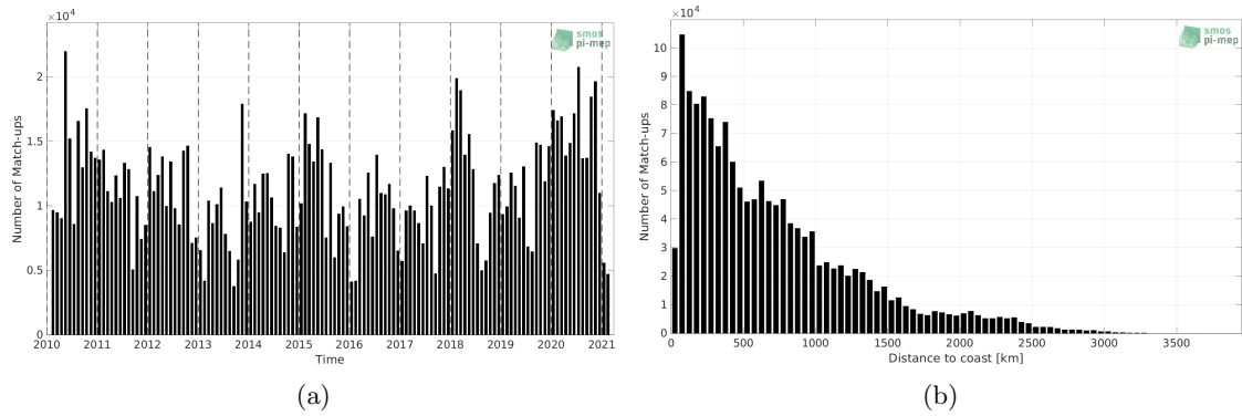
Figure 1: Number of match-ups between TSG (LEGOS-DM) and SMOS SSS L3 v332 - 9 Days (CATDS-CPDC) SSS as a function of time (a) and as function of the distance to coast (b) over the Pacific Ocean Pi-MEP region and for the full satellite product period.
