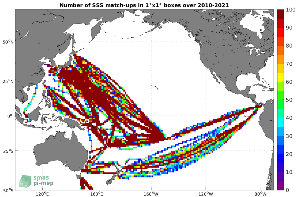
Figure 4: Number of SSS match-ups between TSG (LEGOS-DM) SSS and the SMOS SSS L3 v332 - 9 Days (CATDS-CPDC) SSS product for the Pacific Ocean Pi-MEP region over 1^\circ \times 1^\circ boxes and for the full satellite product period.
