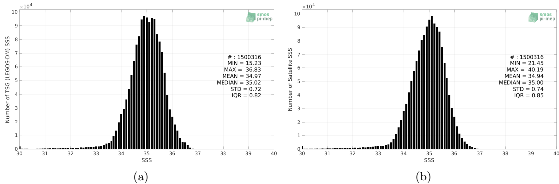
Figure 2: Histograms of SSS from TSG (LEGOS-DM) (a) and SMOS SSS L3 v332 - 9 Days (CATDS-CPDC) (b) considering all match-up pairs per bins of 0.1 over the Pacific Ocean Pi-MEP region and for the full satellite product period.
