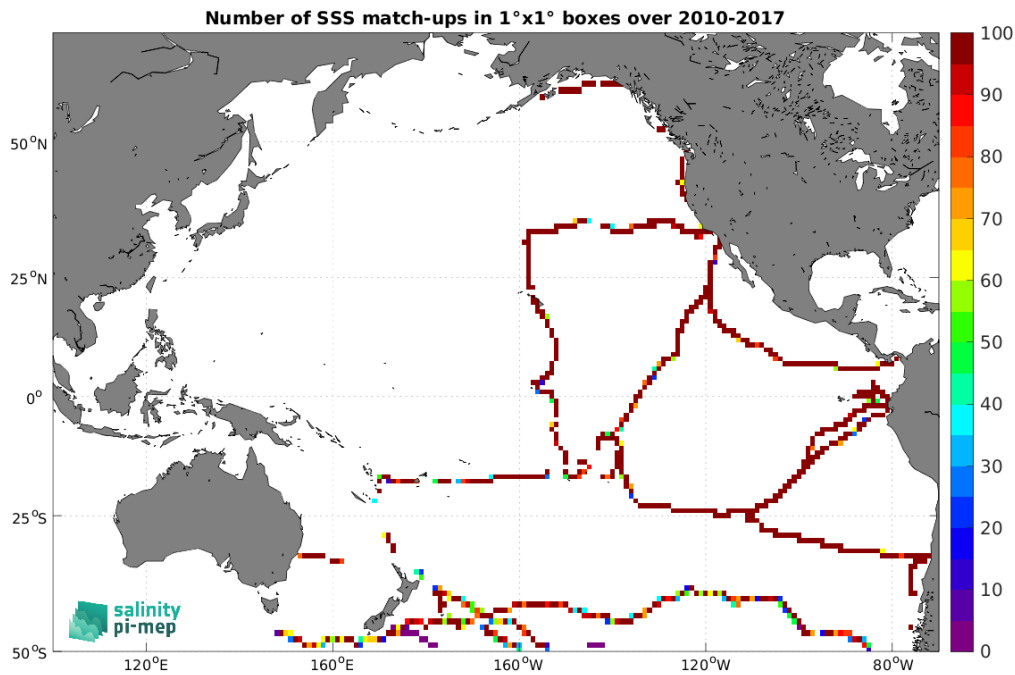
Figure 5: Number of SSS match-ups between TSG (GOSUD-Sailing-ship) SSS and the SMOS SSS L3 v332 - 9 Days (CATDS-CPDC) SSS product for the Pacific Ocean Pi-MEP region over 1^\circ \times 1^\circ boxes and for the full satellite product period.
