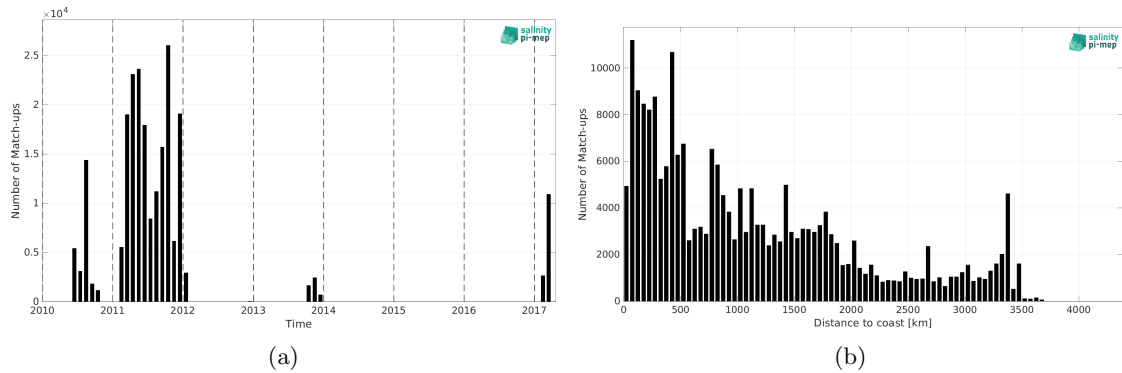
Figure 2: Number of match-ups between TSG (GOSUD-Sailing-ship) and SMOS SSS L3 v332 - 9 Days (CATDS-CPDC) SSS as a function of time (a) and as function of the distance to coast (b) over the Pacific Ocean Pi-MEP region and for the full satellite product period.
