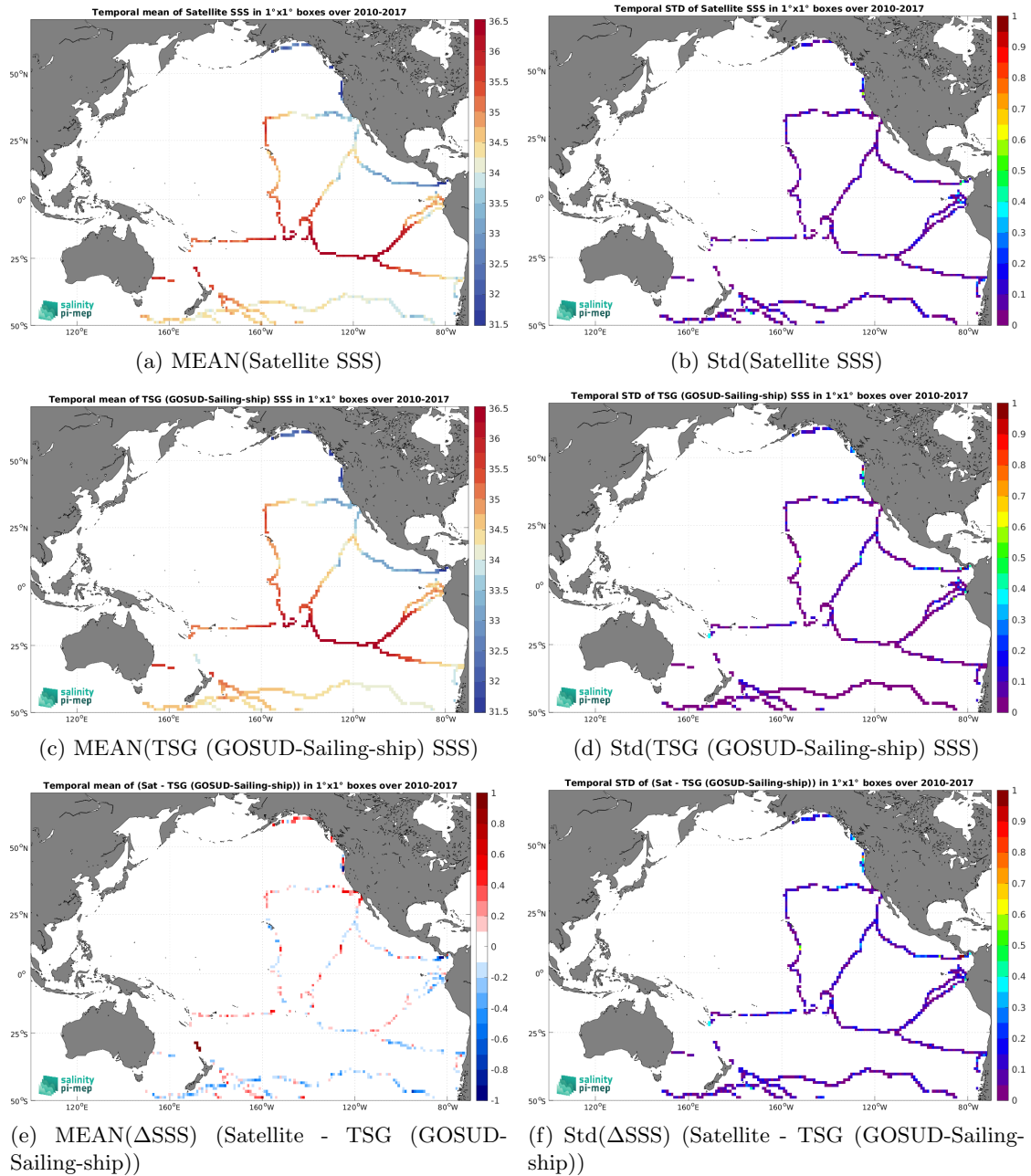
Figure 7: Temporal mean (left) and Std (right) of SSS from SMOS SSS L3 v332 - 9 Days (CATDS-CPDC) (top), TSG (GOSUD-Sailing-ship) (middle), and of \Delta SSS (Satellite - TSG (GOSUD-Sailing-ship)). Only match-up pairs are used to generate these maps.
