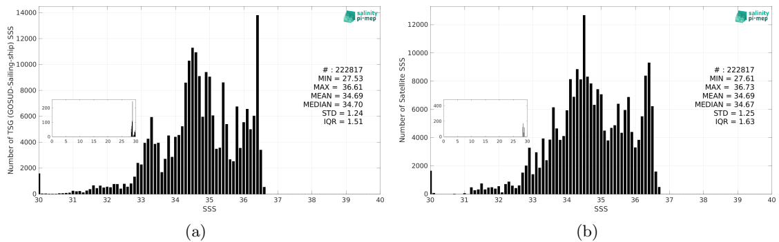
Figure 3: Histograms of SSS from TSG (GOSUD-Sailing-ship) (a) and SMOS SSS L3 v332 - 9 Days (CATDS-CPDC) (b) considering all match-up pairs per bins of 0.1 over the Pacific Ocean Pi-MEP region and for the full satellite product period.
