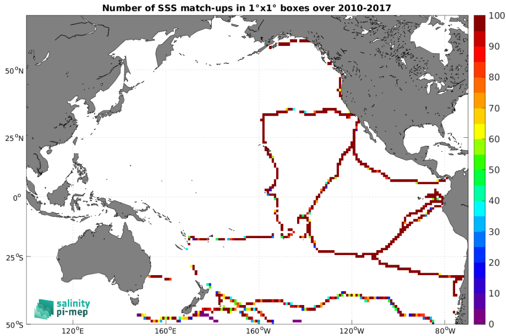
Figure 5: Number of SSS match-ups between TSG (GOSUD-Sailing-ship) SSS and the SMOS SSS L3 v332 - 9 Days (CATDS-CPDC) SSS product for the Pacific Ocean Pi-MEP region over 1°x1° boxes and for the full satellite product period.
