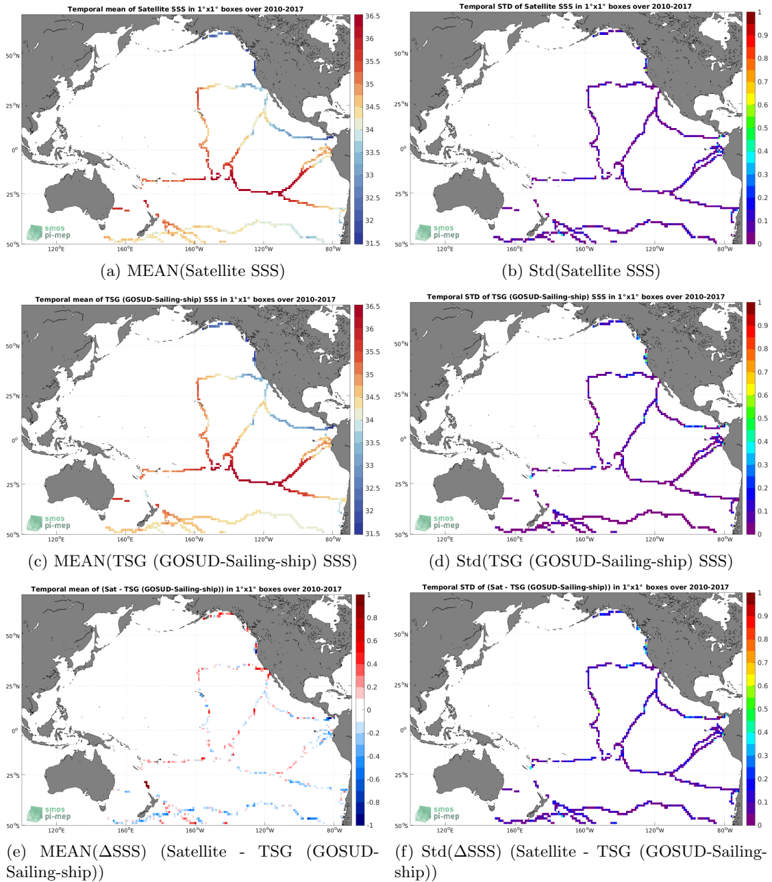
Figure 6: Temporal mean (left) and Std (right) of SSS from SMOS SSS L3 v332 - 9 Days (CATDS-CPDC) (top), TSG (GOSUD-Sailing-ship) (middle), and of \Delta SSS (Satellite - TSG (GOSUD-Sailing-ship)). Only match-up pairs are used to generate these maps.
