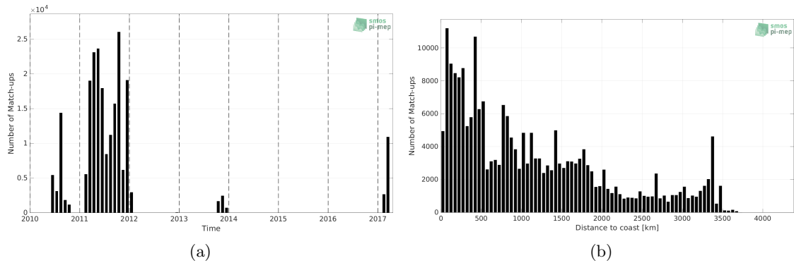
Figure 1: Number of match-ups between TSG (GOSUD-Sailing-ship) and SMOS SSS L3 v332 - 9 Days (CATDS-CPDC) SSS as a function of time (a) and as function of the distance to coast (b) over the Pacific Ocean Pi-MEP region and for the full satellite product period.
