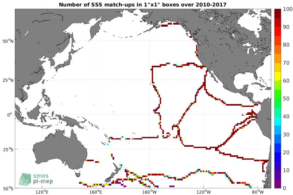
Figure 4: Number of SSS match-ups between TSG (GOSUD-Sailing-ship) SSS and the SMOS SSS L3 v332 - 9 Days (CATDS-CPDC) SSS product for the Pacific Ocean Pi-MEP region over 1^\circ \times 1^\circ boxes and for the full satellite product period.
