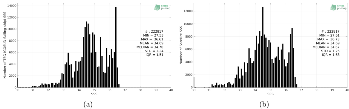
Figure 2: Histograms of SSS from TSG (GOSUD-Sailing-ship) (a) and SMOS SSS L3 v332 - 9 Days (CATDS-CPDC) (b) considering all match-up pairs per bins of 0.1 over the Pacific Ocean Pi-MEP region and for the full satellite product period.
