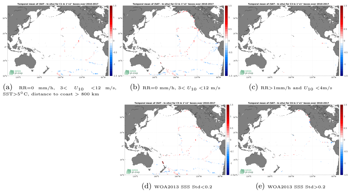
Figure 12: Temporal mean gridded over spatial boxes of size 1^\circ \times 1^\circ of \Delta SSS (SMOS SSS L3 v332 - 9 Days (CATDS-CPDC) - TSG (GOSUD-Sailing-ship)) for 5 different subdatasets corresponding to: RR=0 mm/h, 3 < U_{10} < 12 m/s, SST > 5°C, distance to coast > 800 km (a), RR=0 mm/h, 3 < U_{10} < 12 m/s (b), RR > 1mm/h and U_{10} < 4 m/s (c), WOA2013 SSS Std < 0.2 (d), WOA2013 SSS Std > 0.2 (e).
