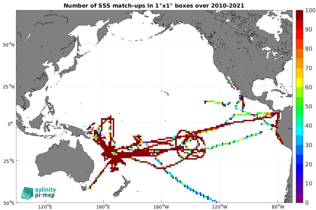
Figure 5: Number of SSS match-ups between TSG (GOSUD-Research-vessel) SSS and the SMOS SSS L3 v332 - 9 Days (CATDS-CPDC) SSS product for the Pacific Ocean Pi-MEP region over 1^\circ \times 1^\circ boxes and for the full satellite product period.
