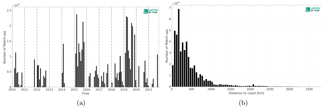
Figure 2: Number of match-ups between TSG (GOSUD-Research-vessel) and SMOS SSS L3 v332 - 9 Days (CATDS-CPDC) SSS as a function of time (a) and as function of the distance to coast (b) over the Pacific Ocean Pi-MEP region and for the full satellite product period.
