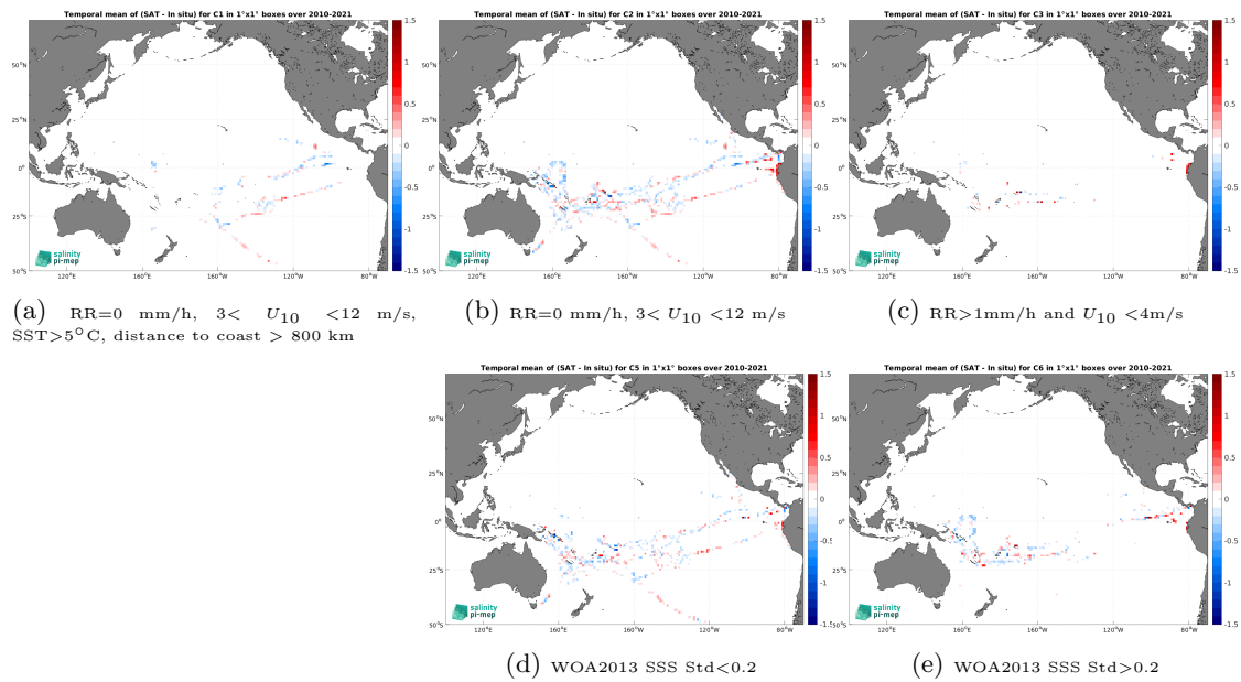
Figure 14: Temporal mean gridded over spatial boxes of size 1^\circ \times 1^\circ of \Delta SSS (SMOS SSS L3 v332 - 9 Days (CATDS-CPDC) - TSG (GOSUD-Research-vessel)) for 5 different subdatasets corresponding to:RR=0 mm/h, 3 < U_{10} < 12 m/s, SST >5^\circ C, distance to coast > 800 km (a), RR=0 mm/h, 3 < U_{10} < 12 m/s (b), RR >1 mm/h and U_{10} < 4 m/s (c), WOA2013 SSS Std <0.2 (d), WOA2013 SSS Std >0.2 (e).
