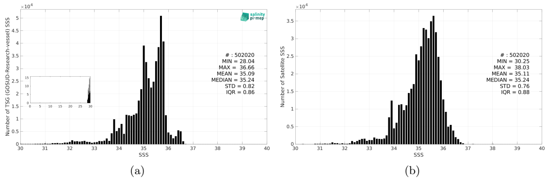
Figure 3: Histograms of SSS from TSG (GOSUD-Research-vessel) (a) and SMOS SSS L3 v332 - 9 Days (CATDS-CPDC) (b) considering all match-up pairs per bins of 0.1 over the Pacific Ocean Pi-MEP region and for the full satellite product period.
