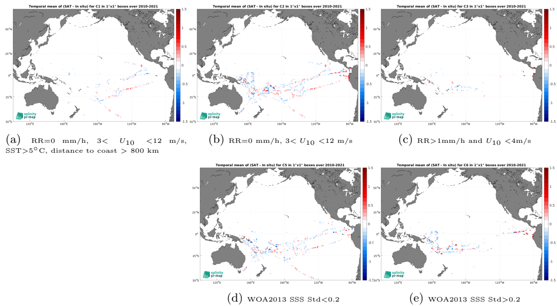
Figure 12: Temporal mean gridded over spatial boxes of size 1^\circ \times 1^\circ of \Delta SSS (SMOS SSS L3 v332 - 9 Days (CATDS-CPDC) - TSG (GOSUD-Research-vessel)) for 5 different subdatasets corresponding to:RR=0 mm/h, 3 < U_{10} < 12 m/s, SST >5^\circ C, distance to coast > 800 km (a), RR=0 mm/h, 3 < U_{10} < 12 m/s (b), RR >1 mm/h and U_{10} < 4 m/s (c), WOA2013 SSS Std <0.2 (d), WOA2013 SSS Std >0.2 (e).
