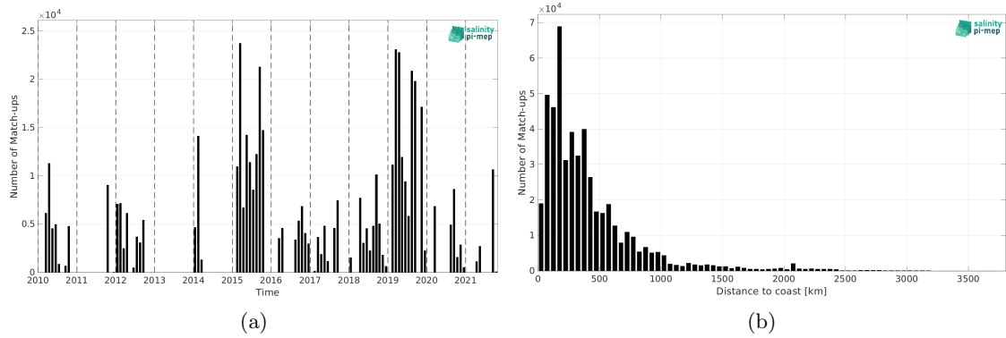
Figure 1: Number of match-ups between TSG (GOSUD-Research-vessel) and SMOS SSS L3 v332 - 9 Days (CATDS-CPDC) SSS as a function of time (a) and as function of the distance to coast (b) over the Pacific Ocean Pi-MEP region and for the full satellite product period.
