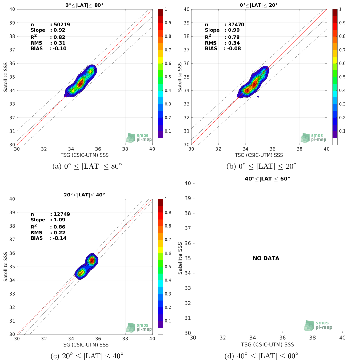
Figure 9: Contour maps of the concentration of SMOS SSS L3 v332 - 9 Days (CATDS-CPDC) SSS (y-axis) versus TSG (CSIC-UTM) SSS (x-axis) at match-up pairs for different latitude bands. For each plot, the red line shows x=y . The black thin and dashed lines indicate a linear fit through the data cloud and the \pm 95\% confidence levels, respectively. The number match-up pairs n , the slope and R^2 coefficient of the linear fit, the root mean square (RMS) and the mean bias between satellite and in situ data are indicated for each latitude band in each plots.
