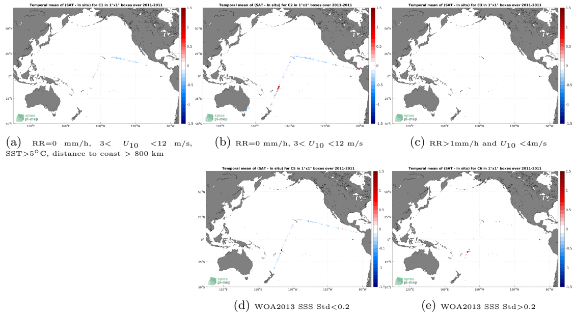
Figure 12: Temporal mean gridded over spatial boxes of size 1^\circ \times 1^\circ of \Delta SSS (SMOS SSS L3 v332 - 9 Days (CATDS-CPDC) - TSG (CSIC-UTM)) for 5 different subdatasets corresponding to:RR=0 mm/h, 3 < U_{10} < 12 m/s, SST >5^\circ C, distance to coast > 800 km (a), RR=0 mm/h, 3 < U_{10} < 12 m/s (b), RR >1 mm/h and U_{10} < 4 m/s (c), WOA2013 SSS Std <0.2 (d), WOA2013 SSS Std >0.2 (e).
