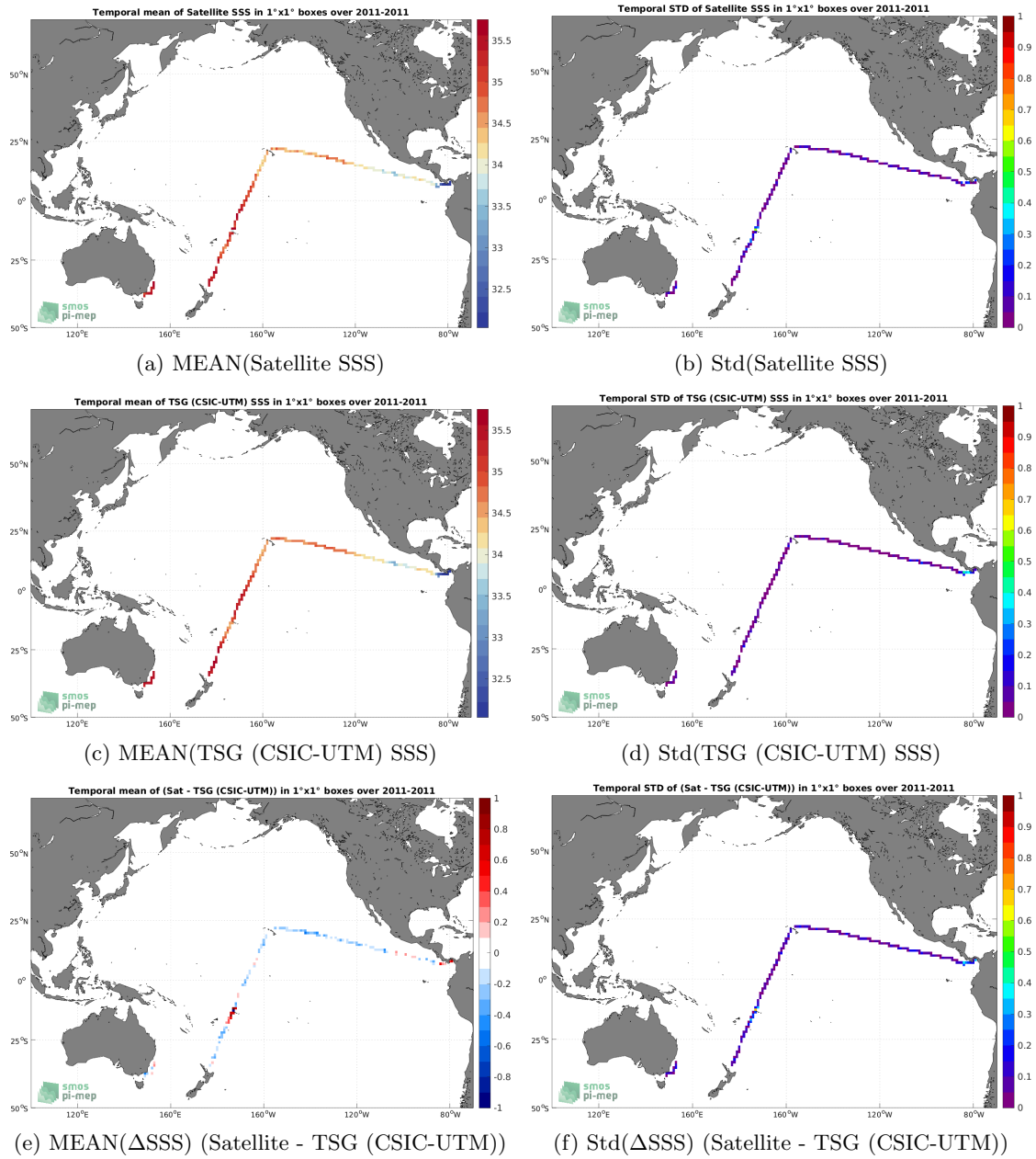
Figure 6: Temporal mean (left) and Std (right) of SSS from SMOS SSS L3 v332 - 9 Days (CATDS-CPDC) (top), TSG (CSIC-UTM) (middle), and of \Delta SSS (Satellite - TSG (CSIC-UTM)). Only match-up pairs are used to generate these maps.
