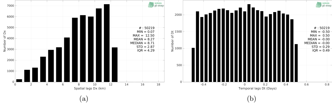
Figure 5: Histograms of the spatial (a) and temporal (b) lags between the location/time of the TSG (CSIC-UTM) measurement and the date of the corresponding SMOS SSS L3 v332 - 9 Days (CATDS-CPDC) SSS pixel.
