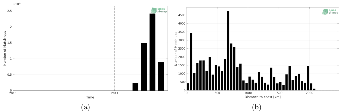
Figure 1: Number of match-ups between TSG (CSIC-UTM) and SMOS SSS L3 v332 - 9 Days (CATDS-CPDC) SSS as a function of time (a) and as function of the distance to coast (b) over the Pacific Ocean Pi-MEP region and for the full satellite product period.
