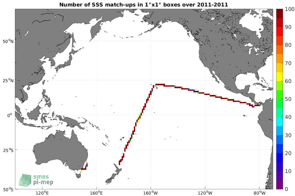
Figure 4: Number of SSS match-ups between TSG (CSIC-UTM) SSS and the SMOS SSS L3 v332 - 9 Days (CATDS-CPDC) SSS product for the Pacific Ocean Pi-MEP region over 1^\circ \times 1^\circ boxes and for the full satellite product period.
