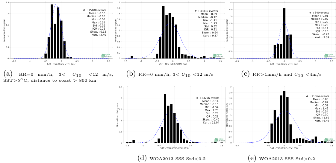
Figure 13: Normalized histogram of \Delta\text{SSS} (SMOS SSS L3 v332 - 9 Days (CATDS-CPDC) - TSG (CSIC-UTM)) for 5 different subdatasets corresponding to: RR=0 mm/h, 3 < U_{10} < 12 m/s, SST>5°C, distance to coast > 800 km (a), RR=0 mm/h, 3 < U_{10} < 12 m/s (b), RR>1mm/h and U_{10} < 4 m/s (c), WOA2013 SSS Std<0.2 (d), WOA2013 SSS Std>0.2 (e).
