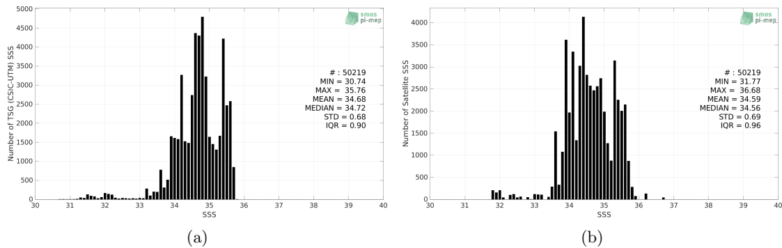
Figure 2: Histograms of SSS from TSG (CSIC-UTM) (a) and SMOS SSS L3 v332 - 9 Days (CATDS-CPDC) (b) considering all match-up pairs per bins of 0.1 over the Pacific Ocean Pi-MEP region and for the full satellite product period.
