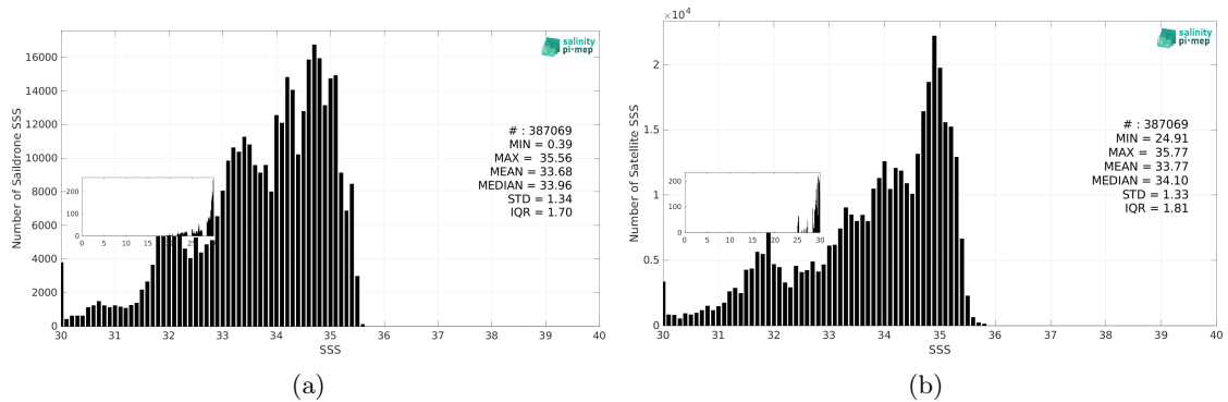
Figure 3: Histograms of SSS from Saildrone (a) and SMOS SSS L3 v332 - 9 Days (CATDS-CPDC) (b) considering all match-up pairs per bins of 0.1 over the Pacific Ocean Pi-MEP region and for the full satellite product period.
