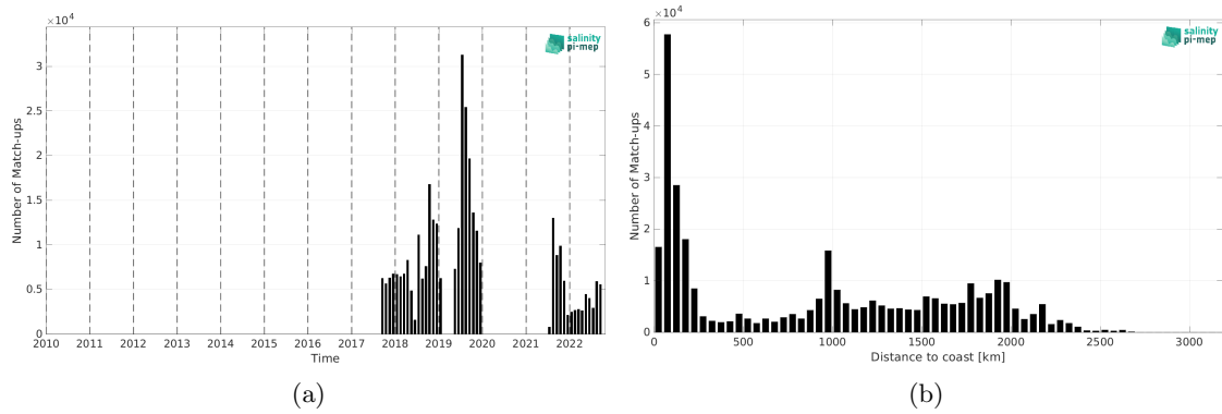
Figure 1: Number of match-ups between Saildrone and SMOS SSS L3 v332 - 9 Days (CATDS-CPDC) SSS as a function of time (a) and as function of the distance to coast (b) over the Pacific Ocean Pi-MEP region and for the full satellite product period.
