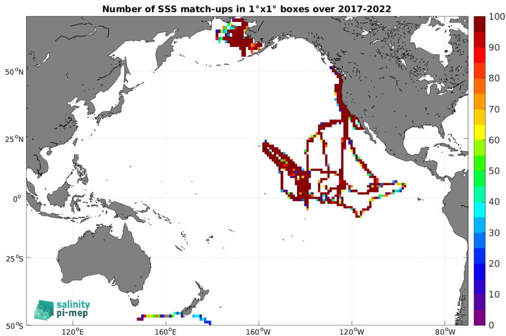
Figure 4: Number of SSS match-ups between Saildrone SSS and the SMOS SSS L3 v332 - 9 Days (CATDS-CPDC) SSS product for the Pacific Ocean Pi-MEP region over 1^\circ \times 1^\circ boxes and for the full satellite product period.
