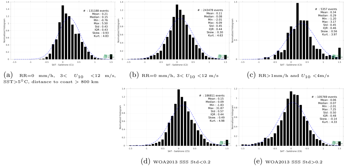
Figure 13: Normalized histogram of \Delta SSS (SMOS SSS L3 v332 - 9 Days (CATDS-CPDC) - Saildrone) for 5 different subdatasets corresponding to: RR=0 mm/h, 3 < U_{10} < 12 m/s, SST >5^{\circ}\text{C} , distance to coast > 800 km (a), RR=0 mm/h, 3 < U_{10} < 12 m/s (b), RR >1 mm/h and U_{10} < 4 m/s (c), WOA2013 SSS Std <0.2 (d), WOA2013 SSS Std >0.2 (e).
