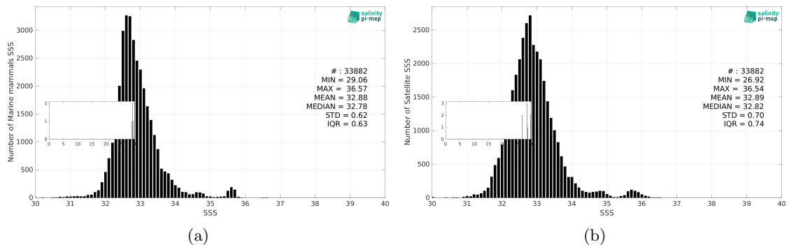
Figure 3: Histograms of SSS from Marine mammals (a) and SMOS SSS L3 v332 - 9 Days (CATDS-CPDC) (b) considering all match-up pairs per bins of 0.1 over the Pacific Ocean Pi-MEP region and for the full satellite product period.
