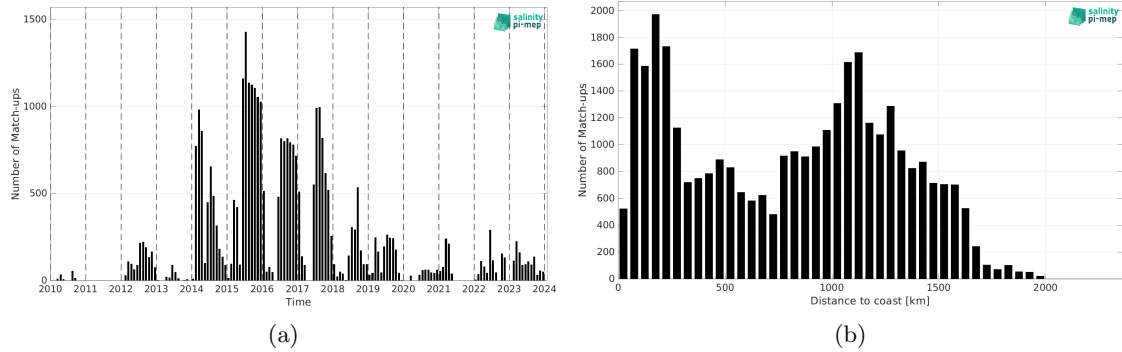
Figure 2: Number of match-ups between Marine mammals and SMOS SSS L3 v332 - 9 Days (CATDS-CPDC) SSS as a function of time (a) and as function of the distance to coast (b) over the Pacific Ocean Pi-MEP region and for the full satellite product period.
