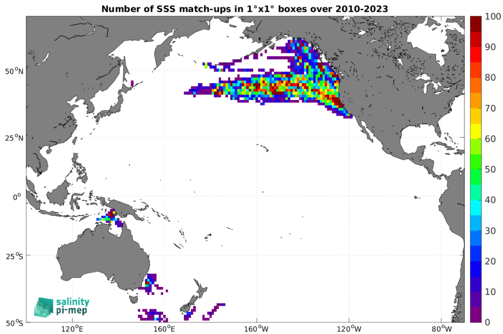
Figure 5: Number of SSS match-ups between Marine mammals SSS and the SMOS SSS L3 v332 - 9 Days (CATDS-CPDC) SSS product for the Pacific Ocean Pi-MEP region over 1^\circ \times 1^\circ boxes and for the full satellite product period.
