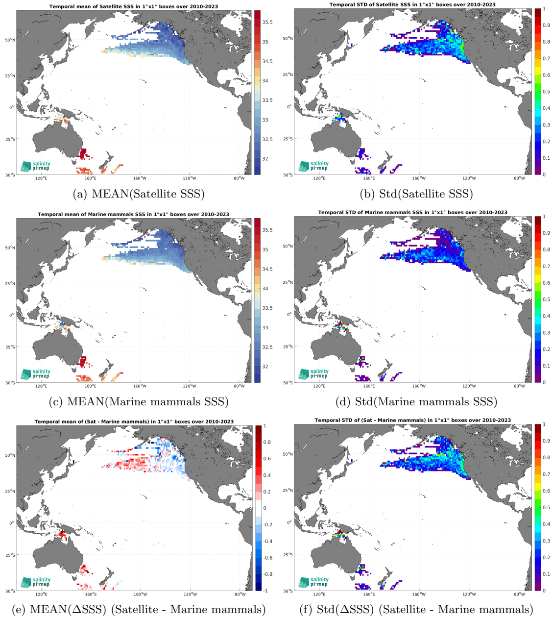
Figure 7: Temporal mean (left) and Std (right) of SSS from SMOS SSS L3 v332 - 9 Days (CATDS-CPDC) (top), Marine mammals (middle), and of \Delta SSS (Satellite - Marine mammals). Only match-up pairs are used to generate these maps.
