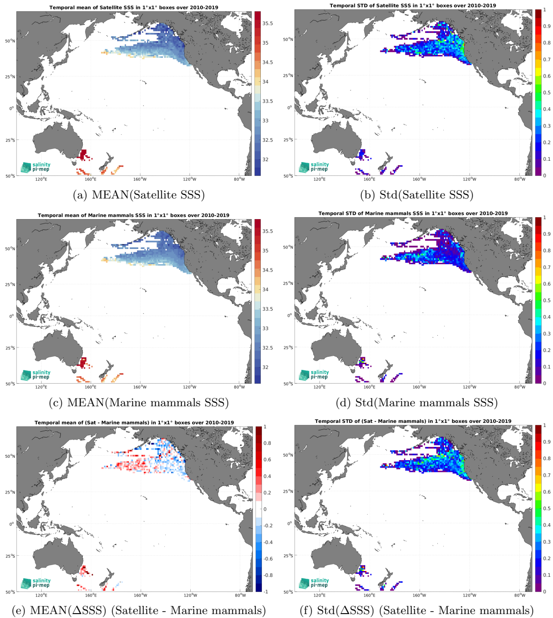
Figure 6: Temporal mean (left) and Std (right) of SSS from SMOS SSS L3 v332 - 9 Days (CATDS-CPDC) (top), Marine mammals (middle), and of \Delta SSS (Satellite - Marine mammals). Only match-up pairs are used to generate these maps.
