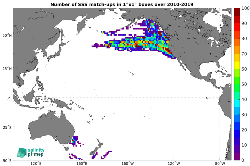
Figure 4: Number of SSS match-ups between Marine mammals SSS and the SMOS SSS L3 v332 - 9 Days (CATDS-CPDC) SSS product for the Pacific Ocean Pi-MEP region over 1^\circ \times 1^\circ boxes and for the full satellite product period.
