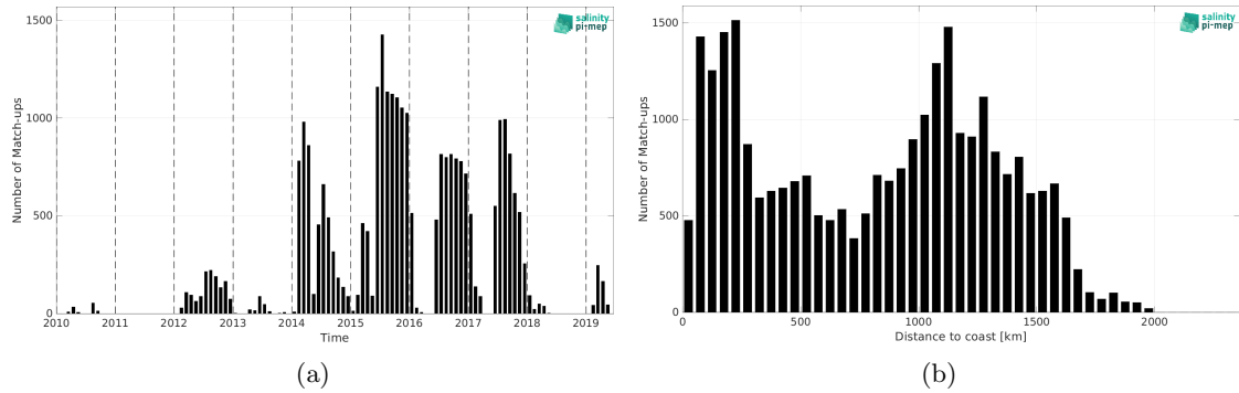
Figure 1: Number of match-ups between Marine mammals and SMOS SSS L3 v332 - 9 Days (CATDS-CPDC) SSS as a function of time (a) and as function of the distance to coast (b) over the Pacific Ocean Pi-MEP region and for the full satellite product period.
