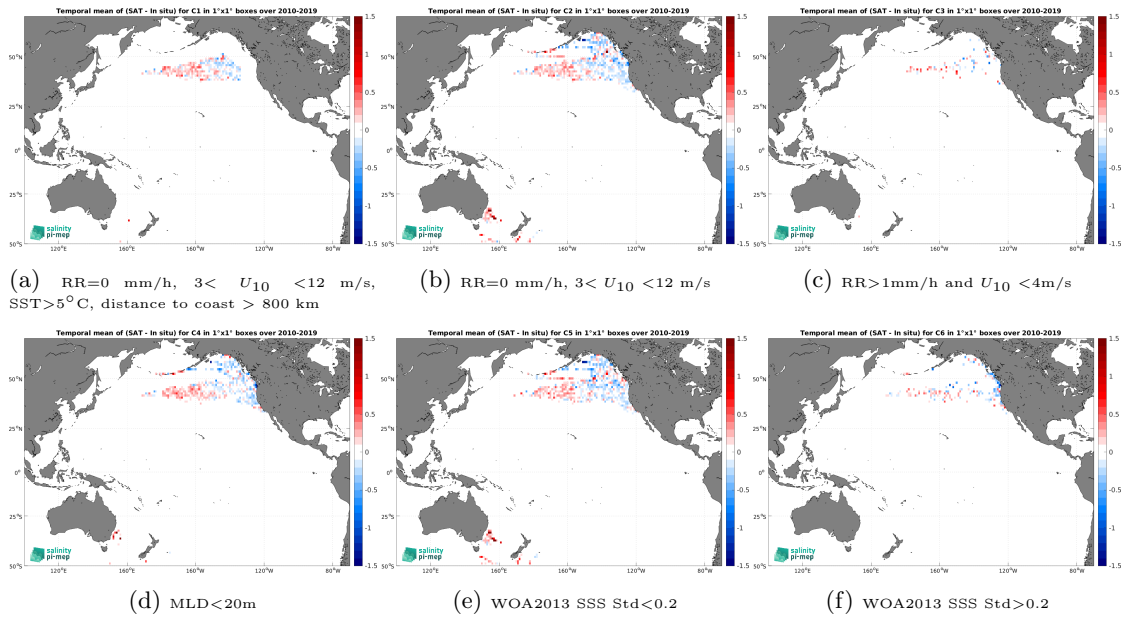
Figure 12: Temporal mean gridded over spatial boxes of size 1^\circ \times 1^\circ of \Delta SSS (SMOS SSS L3 v332 - 9 Days (CATDS-CPDC) - Marine mammals) for 6 different subdatasets corresponding to:RR=0 mm/h, 3 < U_{10} < 12 m/s, SST > 5^\circ\text{C} , distance to coast > 800 km (a), RR=0 mm/h, 3 < U_{10} < 12 m/s (b), RR > 1 mm/h and U_{10} < 4 m/s (c),MLD < 20 m (d),WOA2013 SSS Std < 0.2 (e),WOA2013 SSS Std > 0.2 (f).
