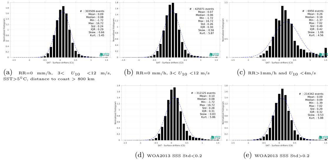
Figure 14: Normalized histogram of \Delta\text{SSS} (SMOS SSS L3 v332 - 9 Days (CATDS-CPDC) - Surface drifters) for 5 different subdatasets corresponding to: RR=0 mm/h, 3 < U_{10} < 12 m/s, SST>5°C, distance to coast > 800 km (a), RR=0 mm/h, 3 < U_{10} < 12 m/s (b), RR>1mm/h and U_{10} < 4 m/s (c), WOA2013 SSS Std<0.2 (d), WOA2013 SSS Std>0.2 (e).
