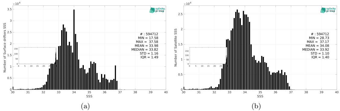
Figure 3: Histograms of SSS from Surface drifters (a) and SMOS SSS L3 v332 - 9 Days (CATDS-CPDC) (b) considering all match-up pairs per bins of 0.1 over the Pacific Ocean Pi-MEP region and for the full satellite product period.
