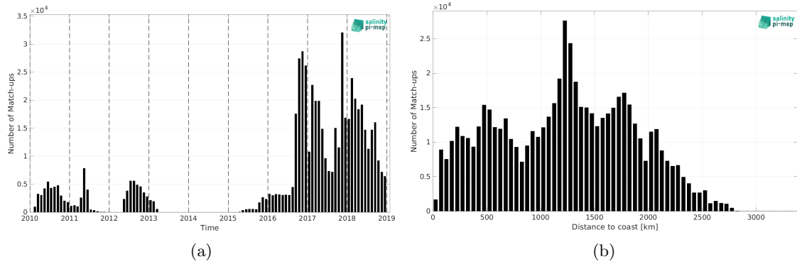
Figure 2: Number of match-ups between Surface drifters and SMOS SSS L3 v332 - 9 Days (CATDS-CPDC) SSS as a function of time (a) and as function of the distance to coast (b) over the Pacific Ocean Pi-MEP region and for the full satellite product period.
