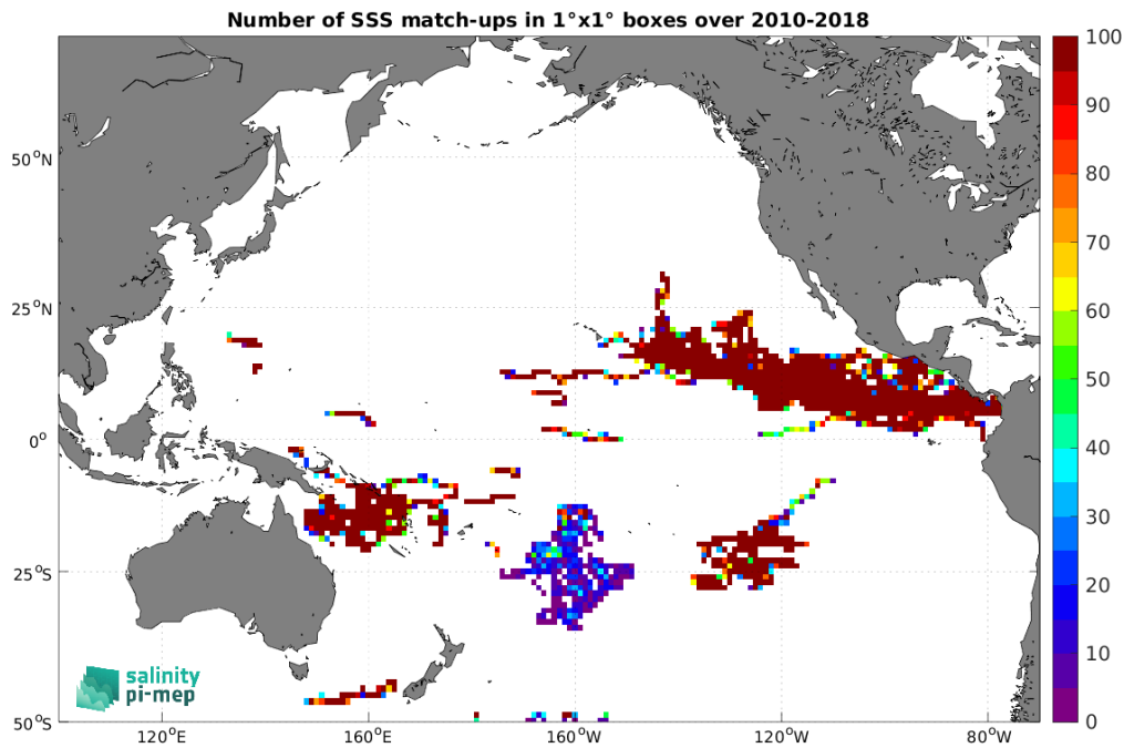
Figure 4: Number of SSS match-ups between Surface drifters SSS and the SMOS SSS L3 v332 - 9 Days (CATDS-CPDC) SSS product for the Pacific Ocean Pi-MEP region over 1^\circ \times 1^\circ boxes and for the full satellite product period.
