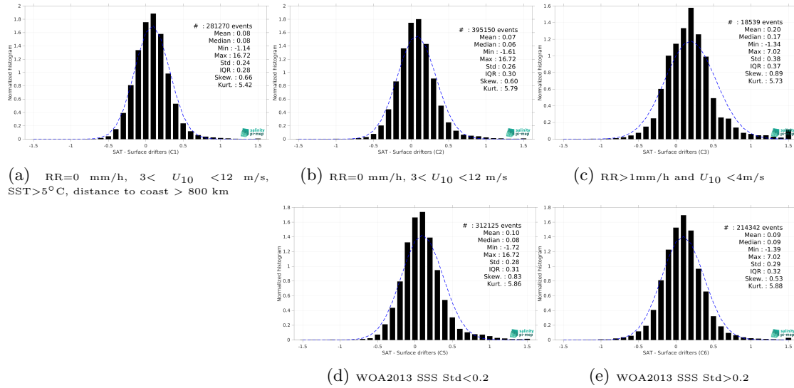
Figure 12: Normalized histogram of \Delta\text{SSS} (SMOS SSS L3 v332 - 9 Days (CATDS-CPDC) - Surface drifters) for 5 different subdatasets corresponding to: RR=0 mm/h, 3 < U_{10} < 12 m/s, SST > 5^\circ\text{C} , distance to coast > 800 km (a), RR=0 mm/h, 3 < U_{10} < 12 m/s (b), RR > 1 mm/h and U_{10} < 4 m/s (c), WOA2013 SSS Std < 0.2 (d), WOA2013 SSS Std > 0.2 (e).
