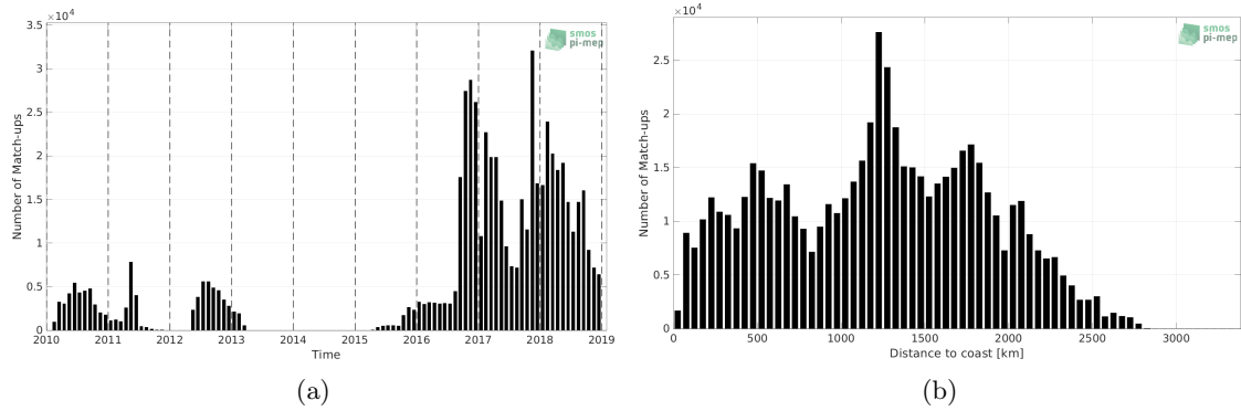
Figure 1: Number of match-ups between Surface drifters and SMOS SSS L3 v332 - 9 Days (CATDS-CPDC) SSS as a function of time (a) and as function of the distance to coast (b) over the Pacific Ocean Pi-MEP region and for the full satellite product period.
