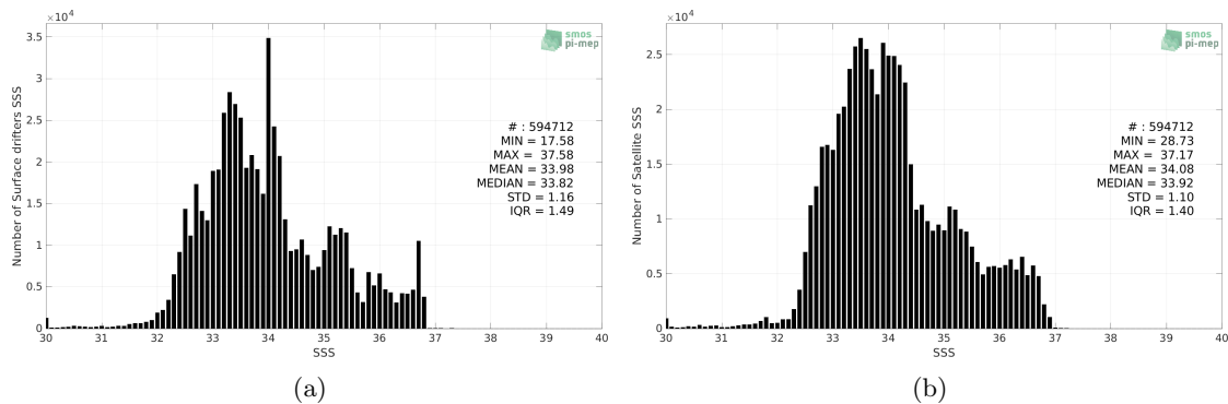
Figure 2: Histograms of SSS from Surface drifters (a) and SMOS SSS L3 v332 - 9 Days (CATDS-CPDC) (b) considering all match-up pairs per bins of 0.1 over the Pacific Ocean Pi-MEP region and for the full satellite product period.
