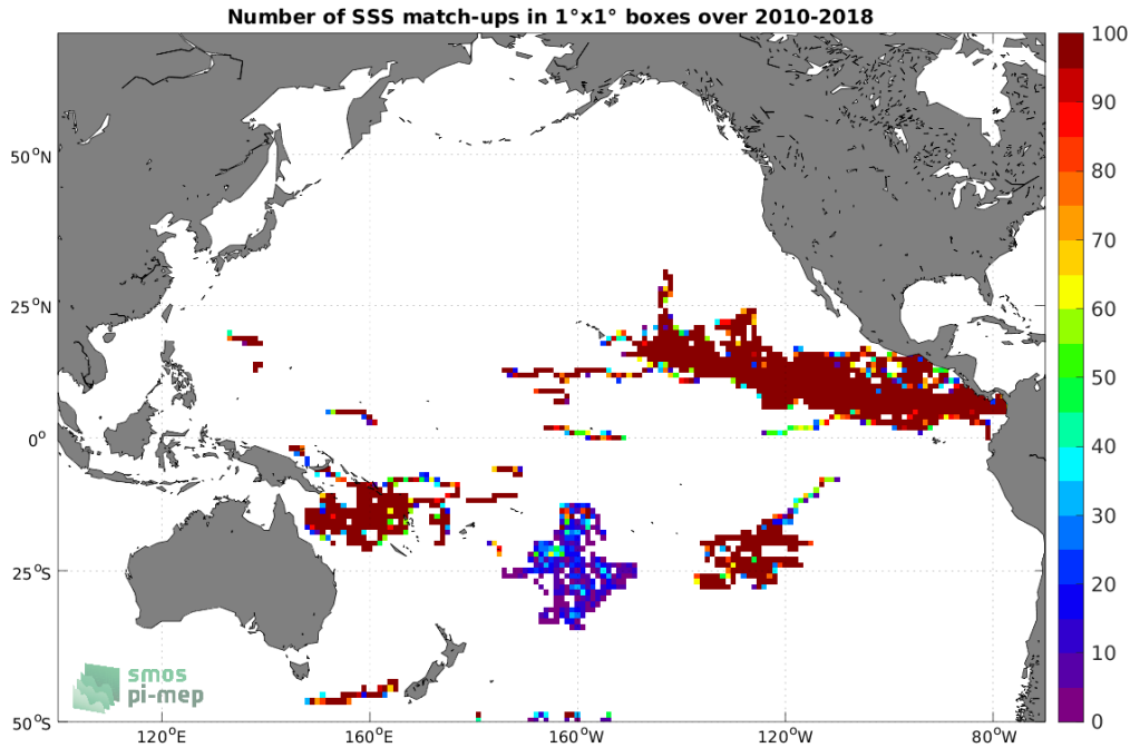
Figure 3: Number of SSS match-ups between Surface drifters SSS and the SMOS SSS L3 v332 - 9 Days (CATDS-CPDC) SSS product for the Pacific Ocean Pi-MEP region over 1^\circ \times 1^\circ boxes and for the full satellite product period.
