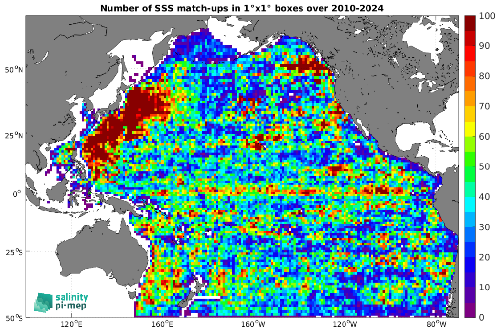
Figure 5: Number of SSS match-ups between Argo SSS and the SMOS SSS L3 v332 - 9 Days (CATDS-CPDC) SSS product for the Pacific Ocean Pi-MEP region over 1^\circ \times 1^\circ boxes and for the full satellite product period.
