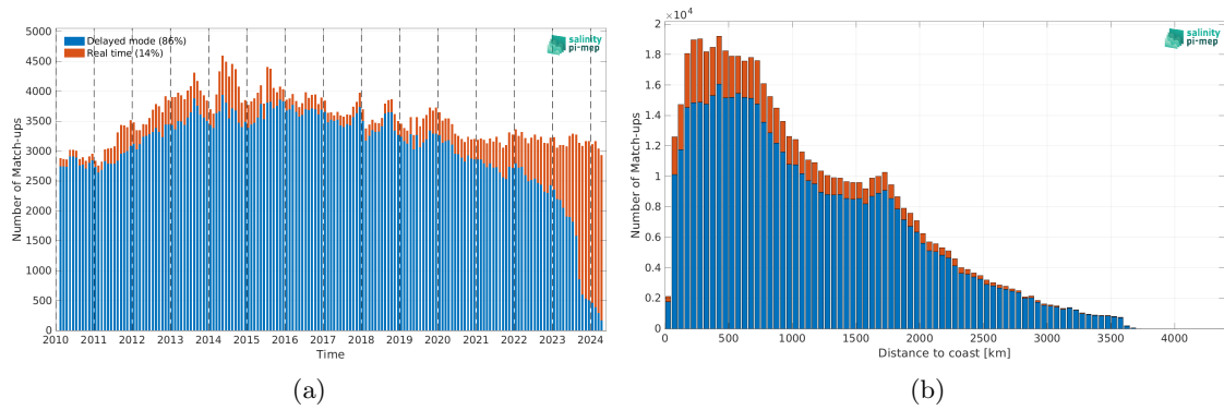
Figure 2: Number of match-ups between Argo and SMOS SSS L3 v332 - 9 Days (CATDS-CPDC) SSS as a function of time (a) and as function of the distance to coast (b) over the Pacific Ocean Pi-MEP region and for the full satellite product period.
