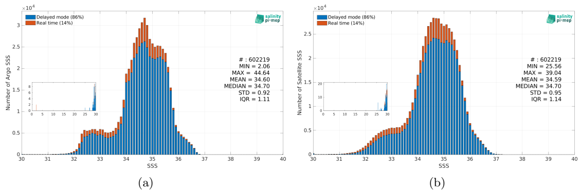
Figure 3: Histograms of SSS from Argo (a) and SMOS SSS L3 v332 - 9 Days (CATDS-CPDC) (b) considering all match-up pairs per bins of 0.1 over the Pacific Ocean Pi-MEP region and for the full satellite product period.
