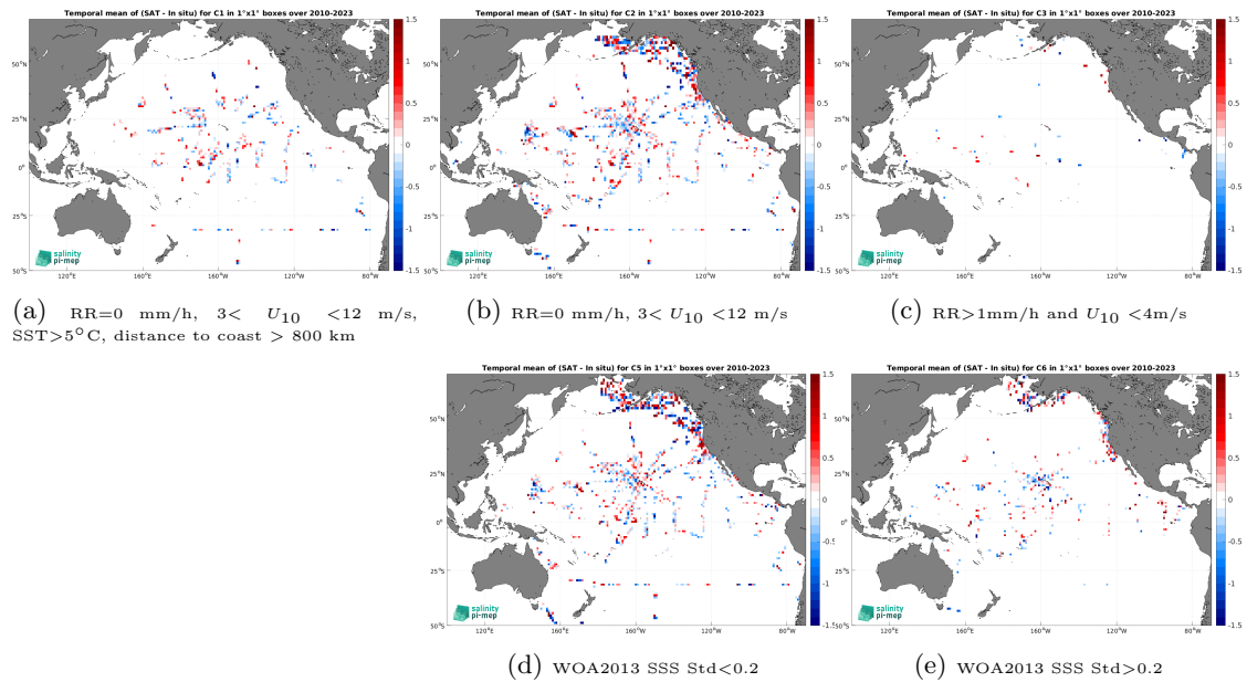
Figure 12: Temporal mean gridded over spatial boxes of size 1^\circ \times 1^\circ of \Delta SSS (SMOS SSS L2Q v331 - 0.25 Deg (CATDS-CPDC) - TSG (SAMOS)) for 5 different subdatasets corresponding to: RR=0 mm/h, 3 < U_{10} < 12 m/s, SST > 5^\circ\text{C} , distance to coast > 800 km (a), RR=0 mm/h, 3 < U_{10} < 12 m/s (b), RR > 1 mm/h and U_{10} < 4 m/s (c), WOA2013 SSS Std < 0.2 (d), WOA2013 SSS Std > 0.2 (e).
