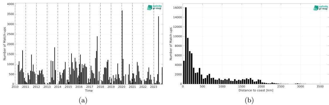
Figure 1: Number of match-ups between TSG (SAMOS) and SMOS SSS L2Q v331 - 0.25 Deg (CATDS-CPDC) SSS as a function of time (a) and as function of the distance to coast (b) over the Pacific Ocean Pi-MEP region and for the full satellite product period.
