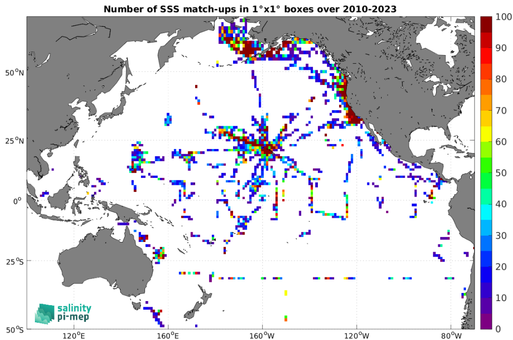
Figure 4: Number of SSS match-ups between TSG (SAMOS) SSS and the SMOS SSS L2Q v331 - 0.25 Deg (CATDS-CPDC) SSS product for the Pacific Ocean Pi-MEP region over 1^\circ \times 1^\circ boxes and for the full satellite product period.
