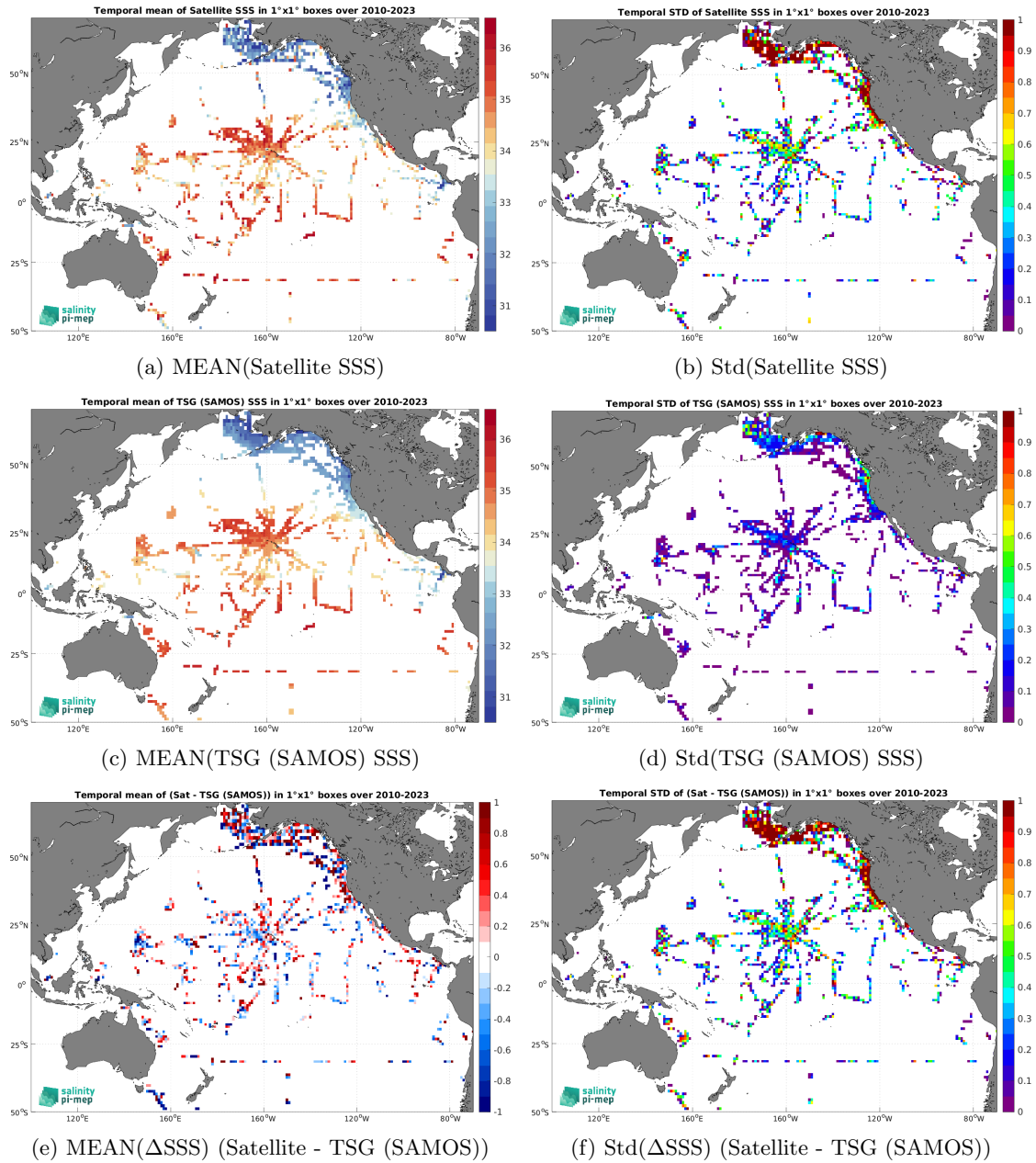
Figure 6: Temporal mean (left) and Std (right) of SSS from SMOS SSS L2Q v331 - 0.25 Deg (CATDS-CPDC) (top), TSG (SAMOS) (middle), and of \Delta SSS (Satellite - TSG (SAMOS)). Only match-up pairs are used to generate these maps.
