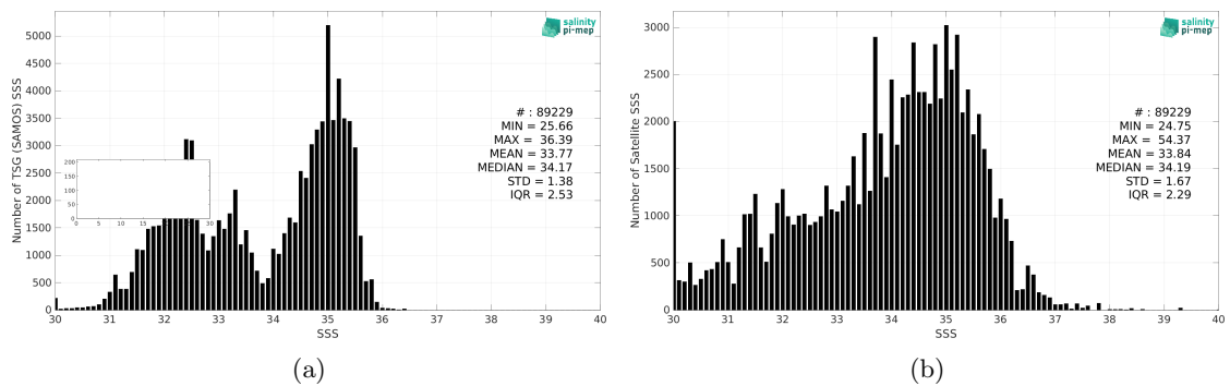
Figure 2: Histograms of SSS from TSG (SAMOS) (a) and SMOS SSS L2Q v331 - 0.25 Deg (CATDS-CPDC) (b) considering all match-up pairs per bins of 0.1 over the Pacific Ocean Pi-MEP region and for the full satellite product period.
