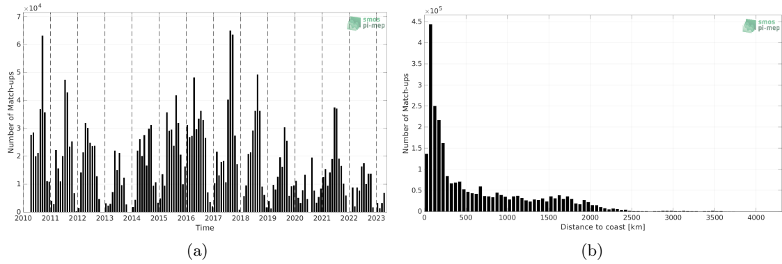
Figure 1: Number of match-ups between TSG (SAMOS) and SMOS SSS L2Q v331 - 0.25 Deg (CATDS-CPDC) SSS as a function of time (a) and as function of the distance to coast (b) over the Pacific Ocean Pi-MEP region and for the full satellite product period.
