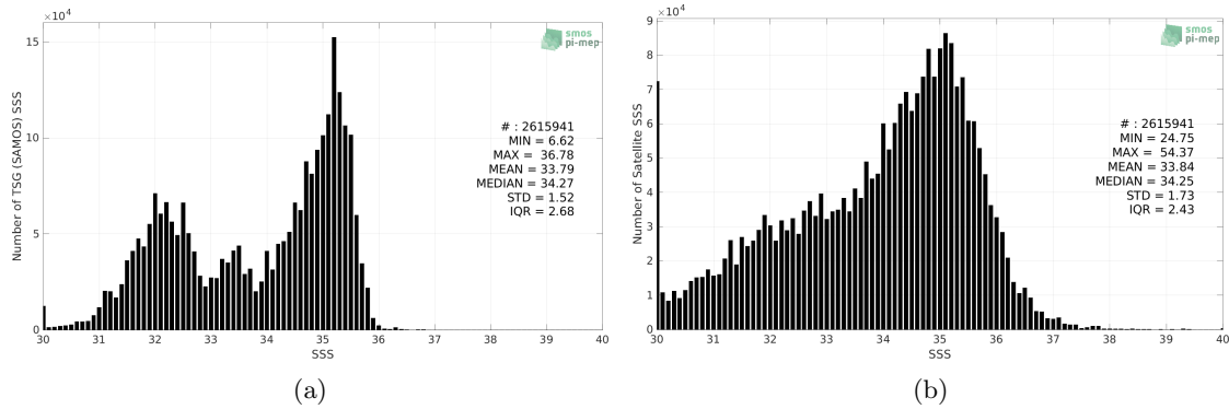
Figure 2: Histograms of SSS from TSG (SAMOS) (a) and SMOS SSS L2Q v331 - 0.25 Deg (CATDS-CPDC) (b) considering all match-up pairs per bins of 0.1 over the Pacific Ocean Pi-MEP region and for the full satellite product period.
