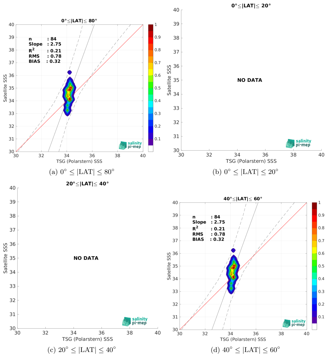
Figure 9: Contour maps of the concentration of SMOS SSS L2Q v331 - 0.25 Deg (CATDS-CPDC) SSS (y-axis) versus TSG (Polarstern) SSS (x-axis) at match-up pairs for different latitude bands. For each plot, the red line shows x=y . The black thin and dashed lines indicate a linear fit through the data cloud and the \pm 95\% confidence levels, respectively. The number match-up pairs n , the slope and R^2 coefficient of the linear fit, the root mean square (RMS) and the mean bias between satellite and in situ data are indicated for each latitude band in each plots.
