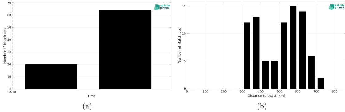
Figure 1: Number of match-ups between TSG (Polarstern) and SMOS SSS L2Q v331 - 0.25 Deg (CATDS-CPDC) SSS as a function of time (a) and as function of the distance to coast (b) over the Pacific Ocean Pi-MEP region and for the full satellite product period.
