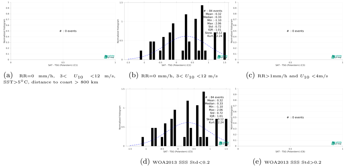
Figure 13: Normalized histogram of \Delta SSS (SMOS SSS L2Q v331 - 0.25 Deg (CATDS-CPDC) - TSG (Polarstern)) for 5 different subdatasets corresponding to: RR=0 mm/h, 3 < U_{10} < 12 m/s, SST>5°C, distance to coast > 800 km (a), RR=0 mm/h, 3 < U_{10} < 12 m/s (b), RR>1mm/h and U_{10} < 4 m/s (c), WOA2013 SSS Std<0.2 (d), WOA2013 SSS Std>0.2 (e).
