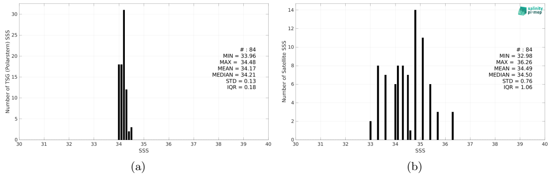
Figure 2: Histograms of SSS from TSG (Polarstern) (a) and SMOS SSS L2Q v331 - 0.25 Deg (CATDS-CPDC) (b) considering all match-up pairs per bins of 0.1 over the Pacific Ocean Pi-MEP region and for the full satellite product period.
