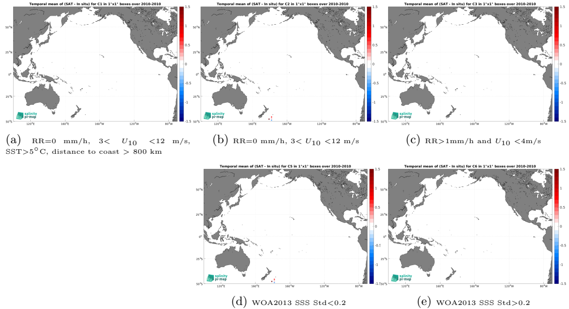
Figure 12: Temporal mean gridded over spatial boxes of size 1^{\circ}\times 1^{\circ} of \Delta\text{SSS} (SMOS SSS L2Q v331 - 0.25 Deg (CATDS-CPDC) - TSG (Polarstern)) for 5 different subdatasets corresponding to:RR=0 mm/h, 3 < U_{10} < 12 m/s, SST >5^{\circ}\text{C} , distance to coast > 800 km (a), RR=0 mm/h, 3 < U_{10} < 12 m/s (b), RR >1 mm/h and U_{10} < 4 m/s (c), WOA2013 SSS Std <0.2 (d), WOA2013 SSS Std >0.2 (e).
