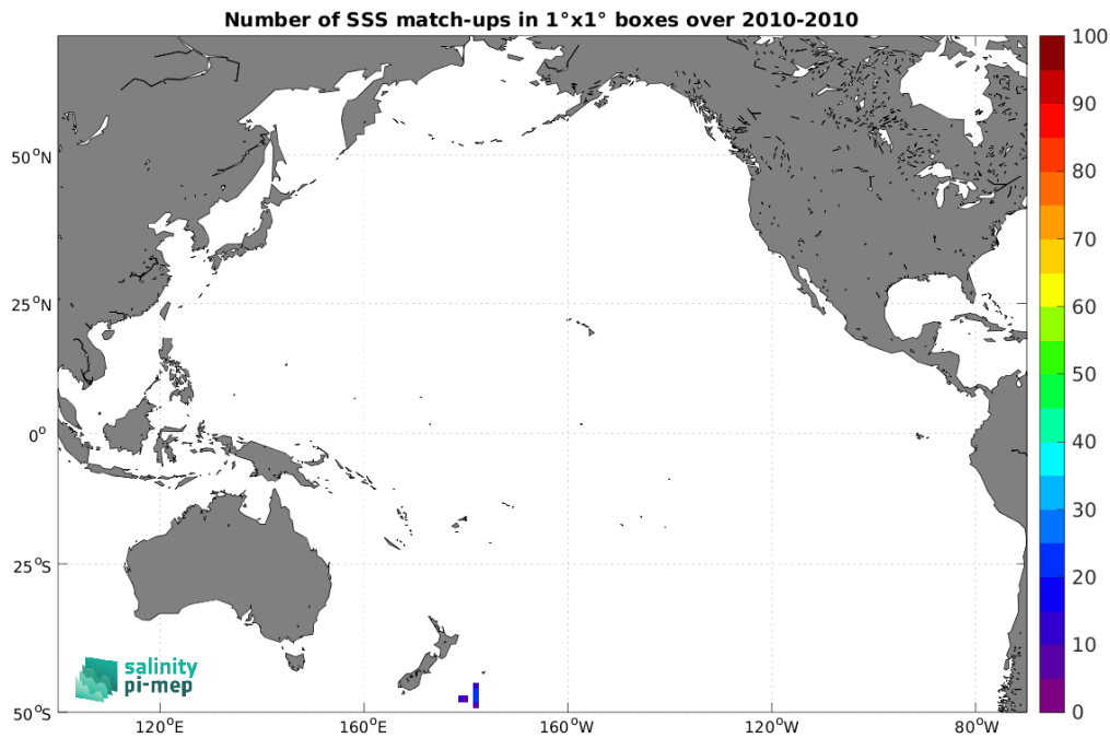
Figure 4: Number of SSS match-ups between TSG (Polarstern) SSS and the SMOS SSS L2Q v331 - 0.25 Deg (CATDS-CPDC) SSS product for the Pacific Ocean Pi-MEP region over 1^\circ \times 1^\circ boxes and for the full satellite product period.
