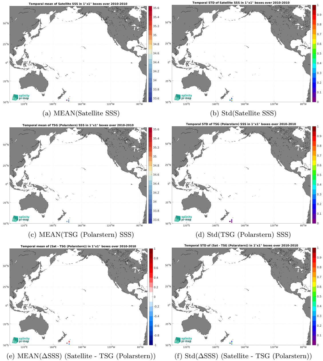
Figure 6: Temporal mean (left) and Std (right) of SSS from SMOS SSS L2Q v331 - 0.25 Deg (CATDS-CPDC) (top), TSG (Polarstern) (middle), and of \Delta SSS (Satellite - TSG (Polarstern)). Only match-up pairs are used to generate these maps.
