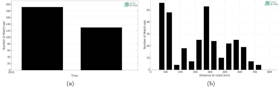
Figure 1: Number of match-ups between TSG (Polarstern) and SMOS SSS L2Q v331 - 0.25 Deg (CATDS-CPDC) SSS as a function of time (a) and as function of the distance to coast (b) over the Pacific Ocean Pi-MEP region and for the full satellite product period.
